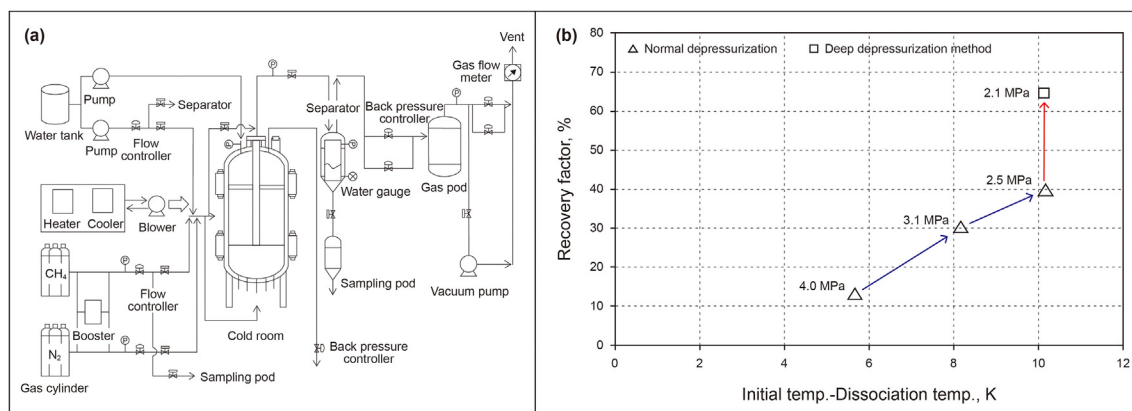
Fig. 10. Physical simulation experiment results of recovery factor (Konno et al., 2014). (a) Schematic diagram of experimental flow; (b) Physical simulation experiment result.
