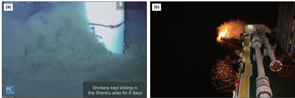
Fig. 7. Two successful gas hydrate production trials in the SCS. (a) Offshore drilling gas hydrate site of the first round trial production (Xinhua News Agency, 2017), (b) The second round trial production site of natural gas hydrate in China's sea area (Trial production site, 2020).
