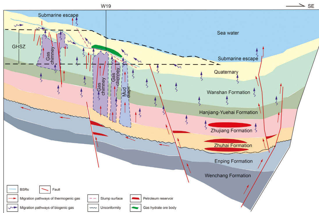
Fig. 5. Gas hydrate accumulation model in the Shenhu Area of the SCS (Zhang and Liang, 2017).
