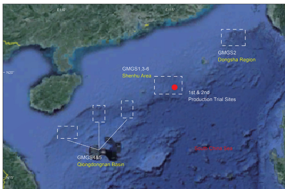
Fig. 2. Location of drilling sites of all drilling expedition during GMGS1–GMGS6 and two production trial sites (Liu and Li, 2021; Wei et al., 2019)
