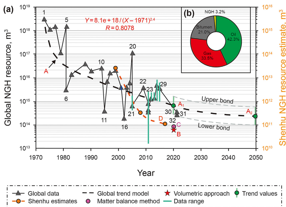
Fig. 1. Estimated results of the global resource of NGH by trend analysis method and compared to other results (Pang et al., 2021): (a) Historical global GIP estimates of NGH showing a general tendency of decreasing resource with time (A), superimposed with fitted statistical trends to project future estimates, projected resource estimates of mode values for RIP of NGH at 2020 and 2050 and their uncertainty range from the statistical trend analysis are added to the plot (A 1 , A 2 ). The estimate of mode value for RIP of NGH from volumetric approach is shown in red star (B) and the average value for the RIP of NGH from matter balance approach is shown in pink dot (C). The historical resource estimates for GIP of NGH from 1999 to 2017 in Shenhu area of SCS are plotted to show the learning curve in brown dotted line (D); (b) The proportion of global TRR of NGH in the total amount of four types of conventional oil and gas resources is shown in the pie chart at the upper right.
