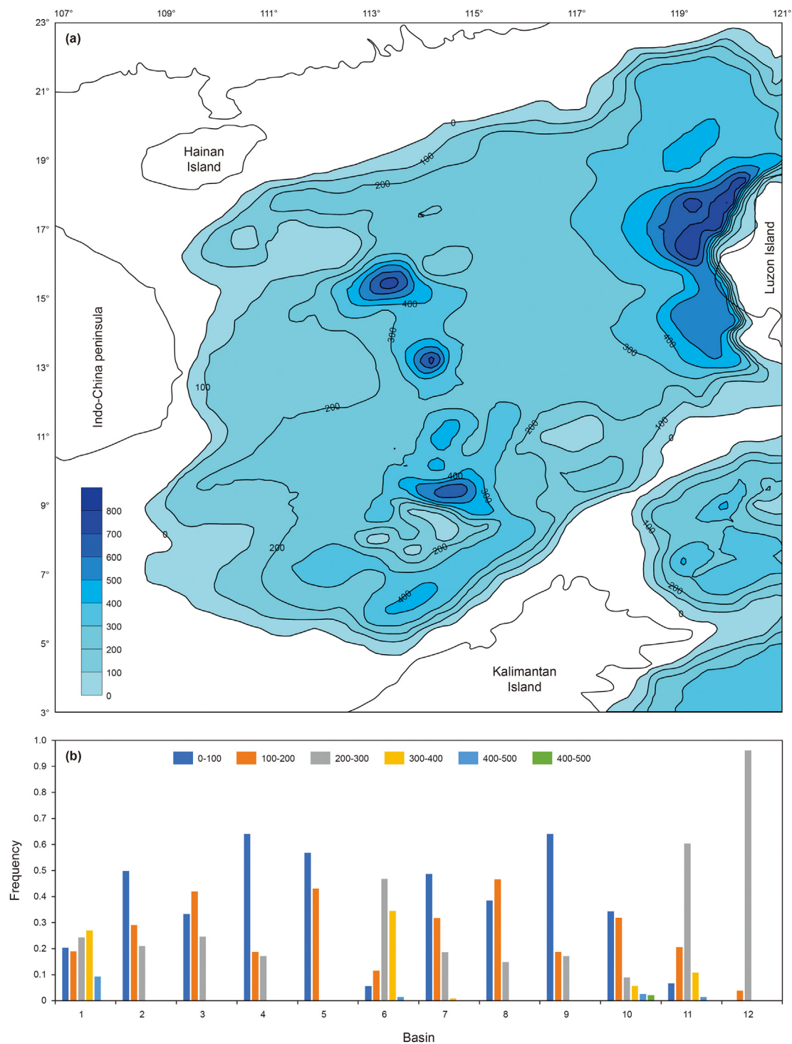
Fig. 4. Predicted stable zones of NGH in the SCS (Xu et al., 2010). (a) Thickness distribution of gas hydrate stable zones in SCS; (b) Statistical chart of NGH stable zone thickness in major basins of the SCS, data source, 1-Southwest Taiwan Basin, 2-Pearl River Mouth Basin, 3-Qiongdongnan Basin, 4-Wan'an Basin, 5-Zengmu Basin, 6-Beikang Basin, 7-Brunei-Sabah Basin, 8-Palawan Basin, 9-Zhongjiannan Basin, 10-Lile Basin, 11-Nanwei Basin, 12-Shuangfeng Basin.
