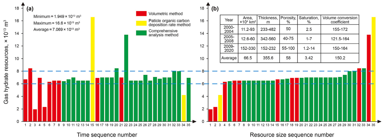
Fig. 6. Evaluation results of NGH resources potential in the SCS over the last twenty years from 2000 to 2020, data from Table 3. (a) Arrange in time order; (b) Arrange in resource size order.
