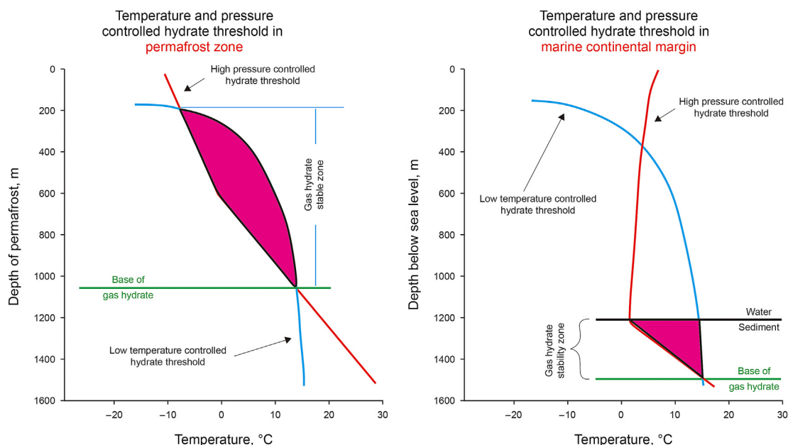
Fig. 8. Diagram of hydrate phase equilibrium model (Modified from Shaibu et al., 2021; Chong and Yang, 2016).
