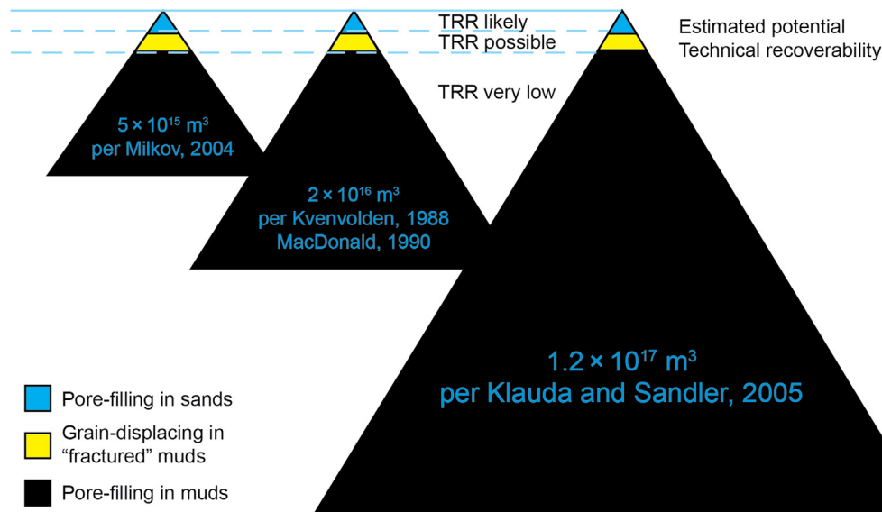
Fig. 9. Enrichment mode diagram of NGH resources (modified from Boswell and Collett, 2006, 2011; Klauda and Sandler, 2005; Kvenvolden, 1988; MacDonald, 1990; Milkov, 2004; Boswell, 2009).
