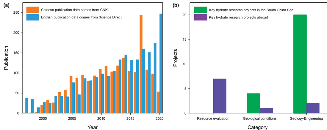
Fig. 3. The number of publications and the key research projects on NGH in China and over the world. (a) The number of Chinese and English publications on gas hydrate in the SCS (the data of Chinese publications are from CNKI; the data of English publications are from Science Direct); (b) Comparison of the research fields involved in the hydrate research projects funded by the Chinese government and by foreign governments (data source Tables 1 and 2).
