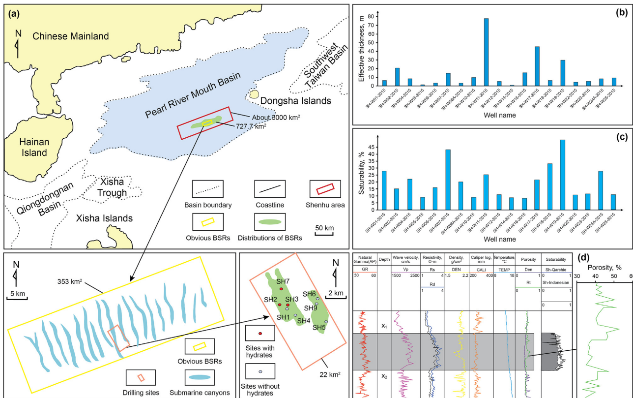
Fig. 11. Location and exploration results of gas hydrate reservoir in the Shenhu Area, Pearl River Mouth Basin, SCS. (Pang et al., 2021). (a) The location of Shenhu area and the prediction results of favorable area for NGH development, modified from Su et al., 2014; the Shenhu Area predicted by seismic data (red frame area 3000 km 2 ); the favorable production area determined after drilling 19 wells (22 km 2 ). (b) Effective thickness of NGH reservoir in 2015, data reference (Yang et al., 2017). (c) NGH saturation, data reference (Yang et al., 2017). (d) NGH porosity of W2 well in the Shenhu Area in 2007, data references (Wang et al., 2010b; Lu et al., 2008).
