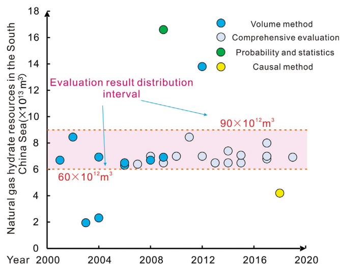
Fig. 2. Assessment results of NGH resources in South China Sea from 2000 to 2020 (modified from Pang et al., 2021).
