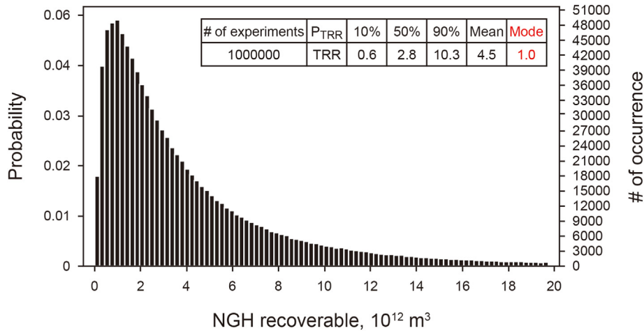
Fig. 9. Monte Carlo simulation results of recoverable natural gas hydrate resources in the South China Sea.
