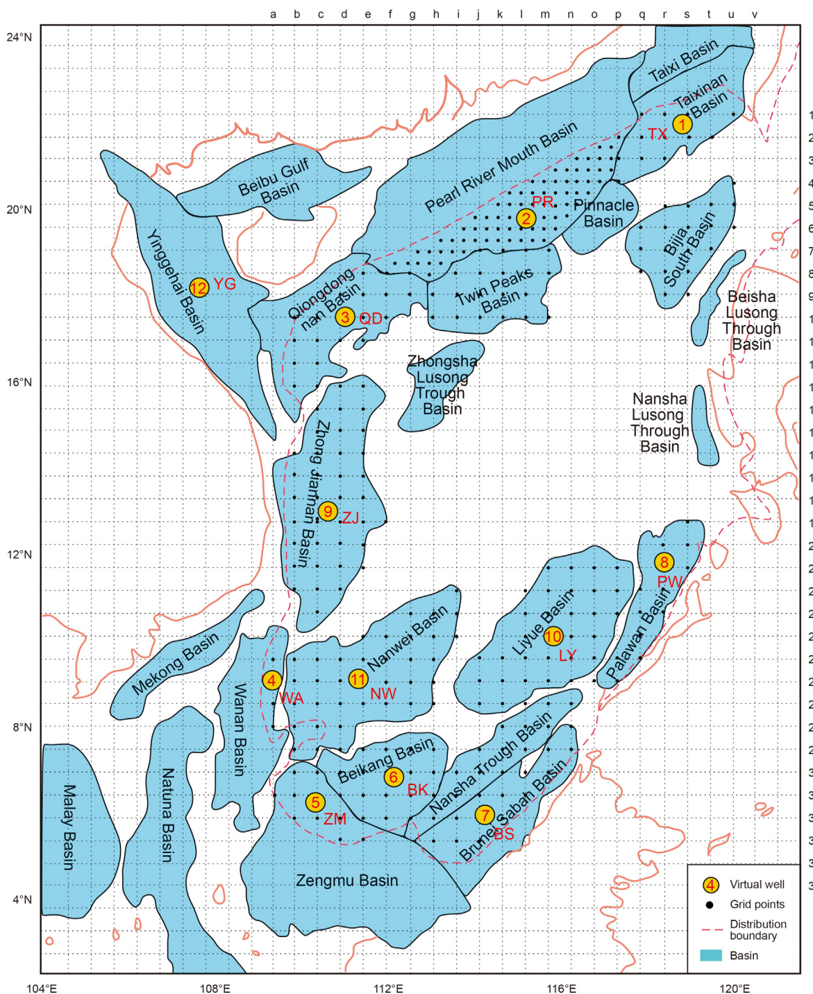
Fig. 3. Overview of the main sedimentary basins and virtual well points in the South China Sea (modified from Feng et al., 2018).
