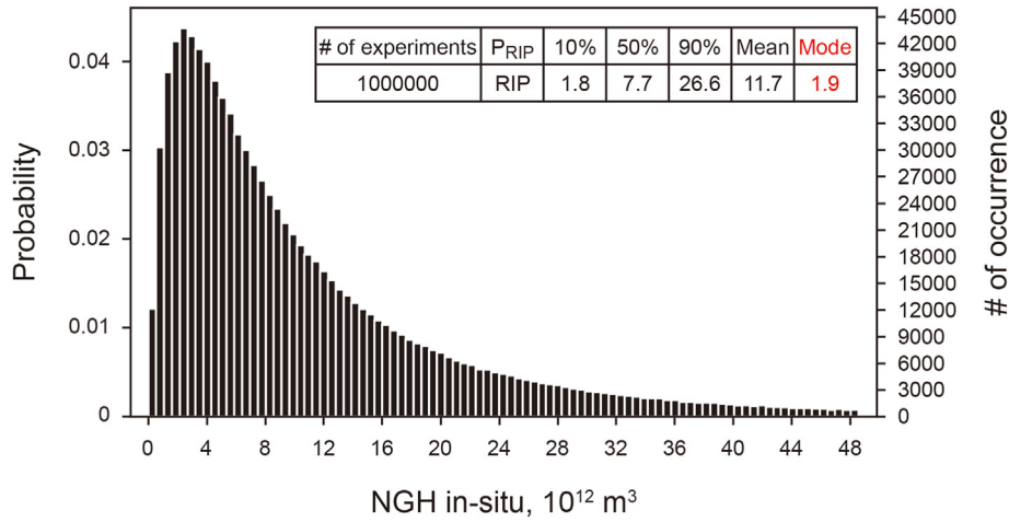
Fig. 8. Monte Carlo simulation results of in-situ natural gas hydrate resources in the South China Sea.
