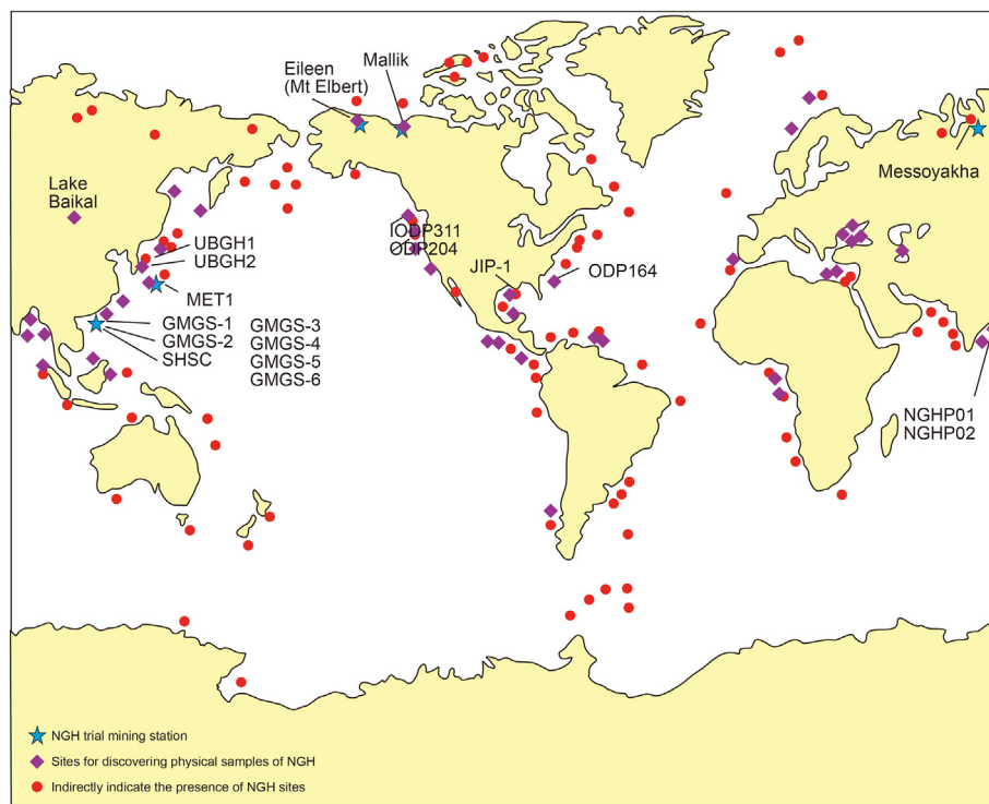
Fig. 1. Distribution of main geological surveys and exploration activities related to natural gas hydrate in the world (modified from Sha et al., 2019).
