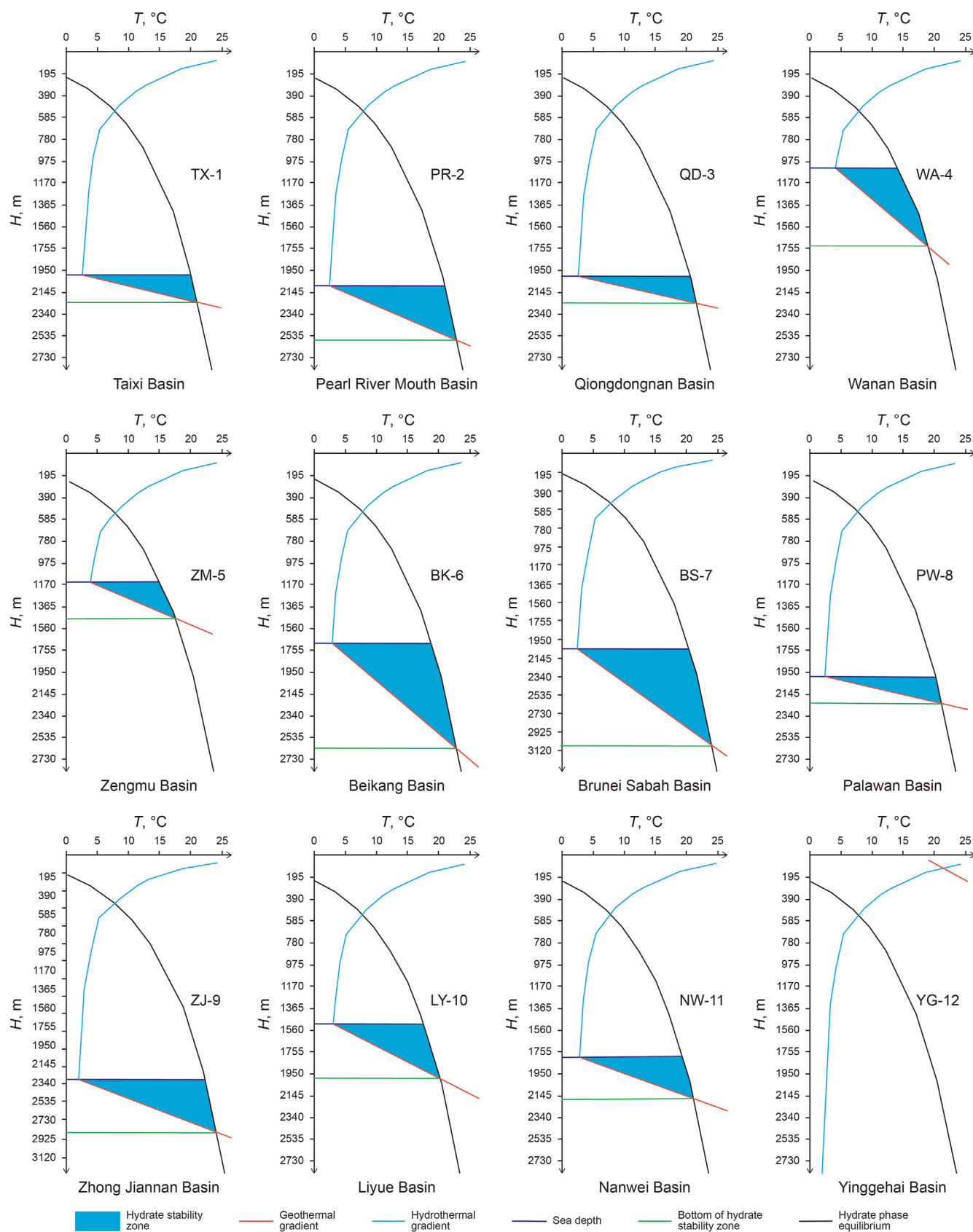
Fig. 4. Distribution characteristics of hydrate phase equilibrium at virtual well points in 12 main basins in the South China Sea.
