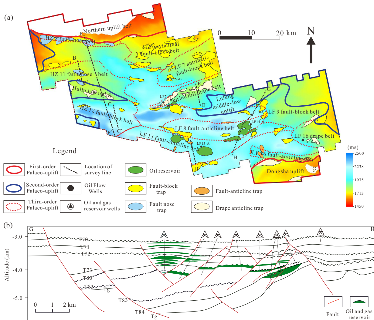
Fig. 3. Distribution map of palaeo-uplifts, traps and reservoirs in the Lufeng Depression.
