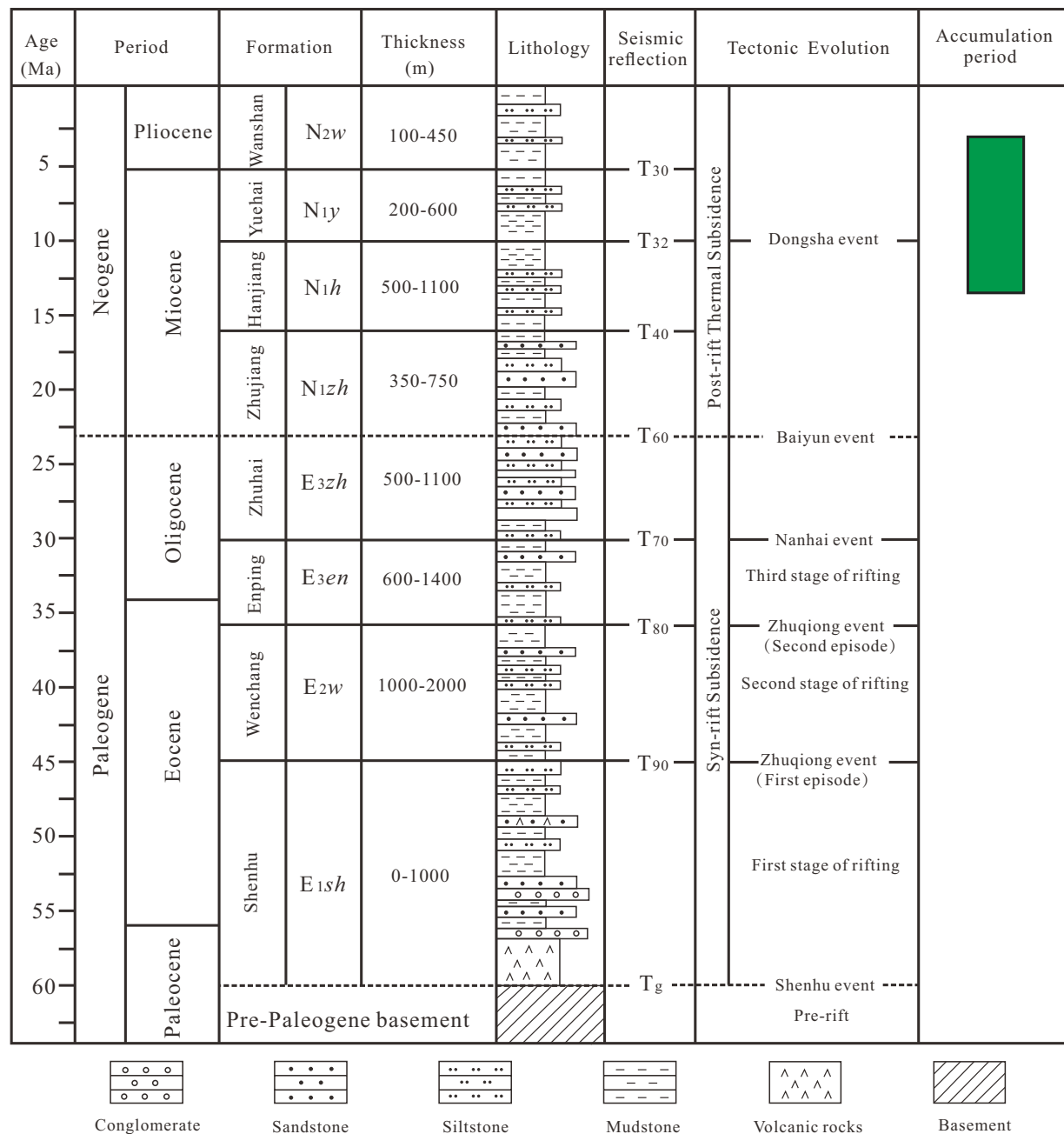
Fig. 2. Stratigraphic histogram of the Lufeng Depression (modified after Yan (2016)).
