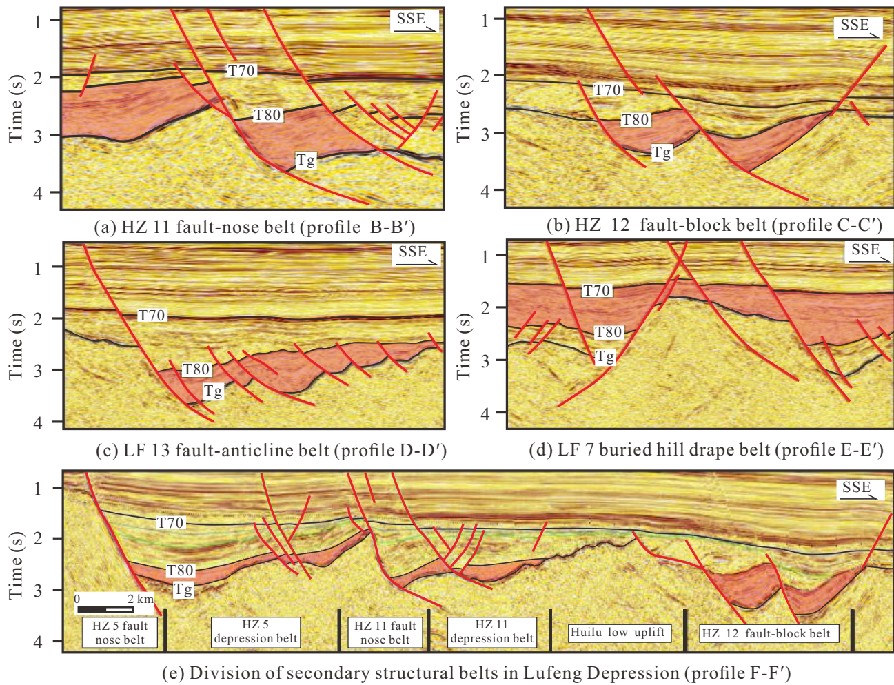
Fig. 4. Types of the main palaeo-uplift structural belts in the Lufeng Depression (for section locations, see Fig. 3).
