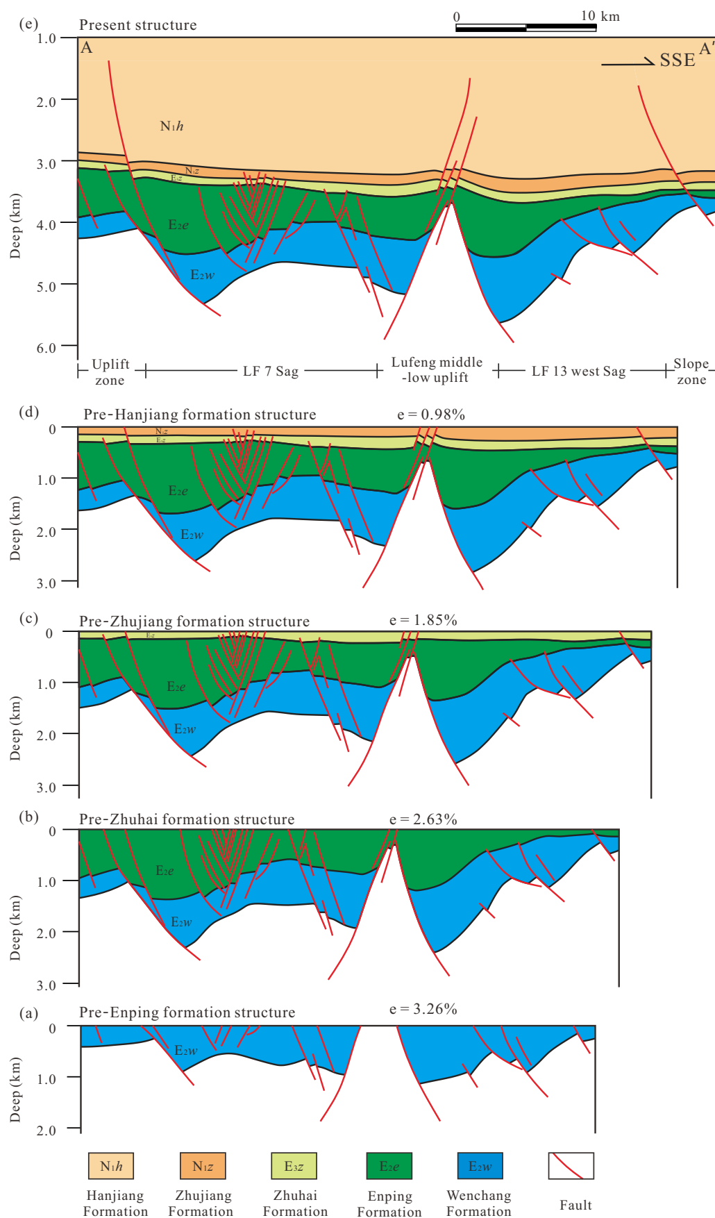
Fig. 5. Structural evolution profile (for section locations, see Fig. 1).
