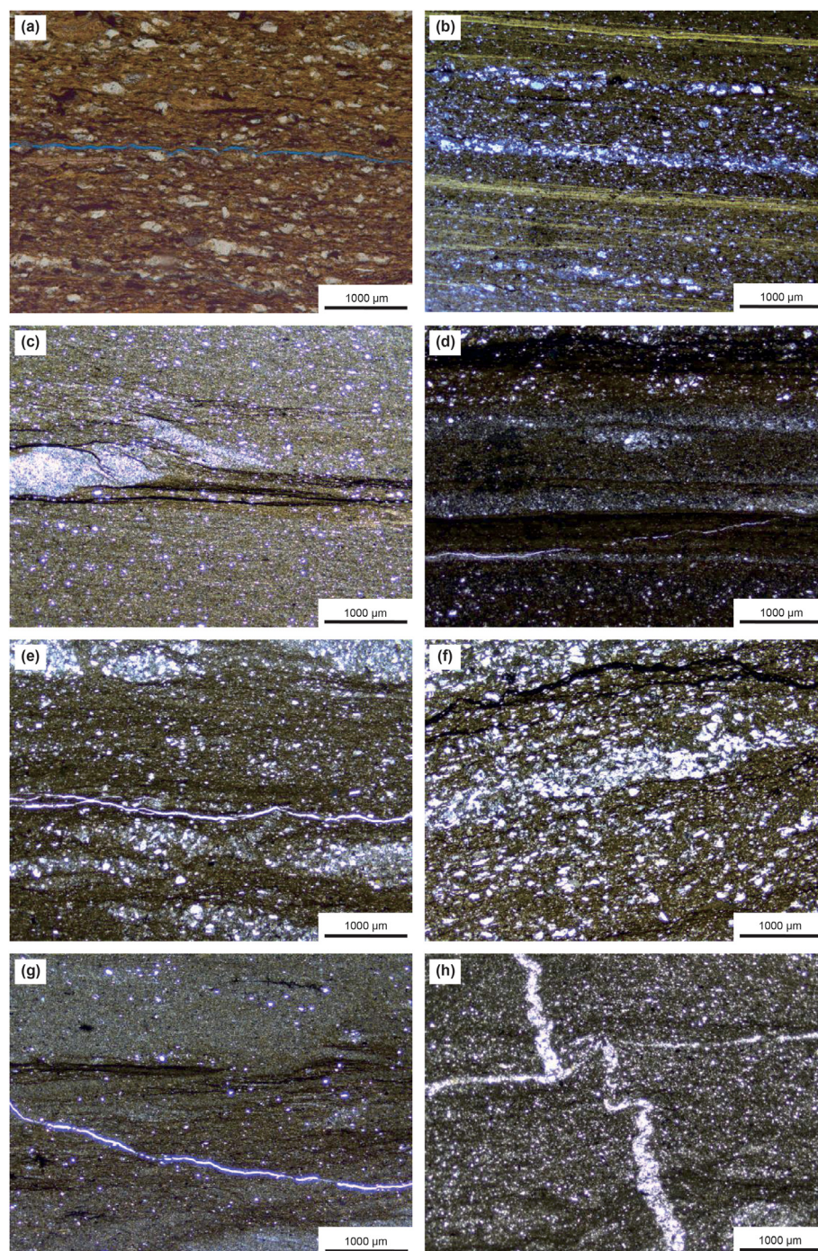
Fig. 3. Thin section images show the bedding fractures in Lucaogou Formation, Jimusar Sag. (a). Micro-fracture parallel to bedding, J176, 3027.29m. (b). Micro-fracture parallel to bedding, J10016, 3310.8m. (c). Filled micro-fractures parallel to bedding planes, J10016, 3311.3m. (d). Half-filled micro-fractures parallel to bedding planes, J251, 3601.065m. (e). Filled micro-fractures parallel to bedding planes, J10016, 3306.3m. (f). Filled micro-fractures parallel to bedding planes, J10016, 3309.2m. (g). Micro-fractures cut through the bedding planes, J10016, 3311.3. (h). Micro-fractures cut through the bedding planes, J10016, 3320.0m.
