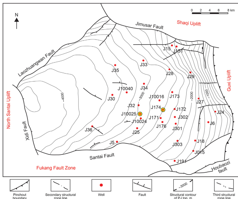
Fig. 1. Map showing structure contour of top of the Lucaogou Formation of the Jimusar Sag in Junggar Basin, West China (S Zhang et al., 2019).
