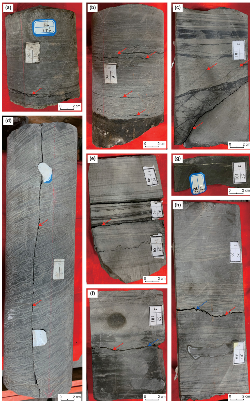
Fig. 2. Core photos show the bedding fractures in Lucaogou Formation, Jimusar Sag. (a). Jagged bedding fractures, J10012, 3293.01m. (b). Three distinct bedding fractures parallel to bedding planes, J10012, 3294.13m. (c). Inclined fractures, J10016. (d). Vertical fractures, J10012. (e). Minerals filling in the bedding planes, J10016. (f). Dissolution and cementation along the bedding surfaces, J10016. (g). Pyrite filling in the bedding planes, J10016. (h). Dissolution and cementation along the bedding surfaces, J10016.
