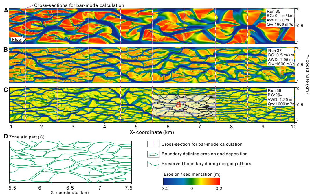
Fig. 7. Bar morphology in modelled braided rivers with varying bed gradients and fixed discharge ( 1600 \text{ m}^3/\text{s} ). AWD, average water depth; BG, bed gradient; Qw, flow discharge. (A) to (C) Maps of riverbed erosion and sedimentation produced by different runs, with bed gradients of 0.1 \text{ m/km} , 0.5 \text{ m/km} and 2.0 \text{ m/km} , respectively. (D) Bar boundaries extracted from the part of map corresponding to Zone A in part (D).
