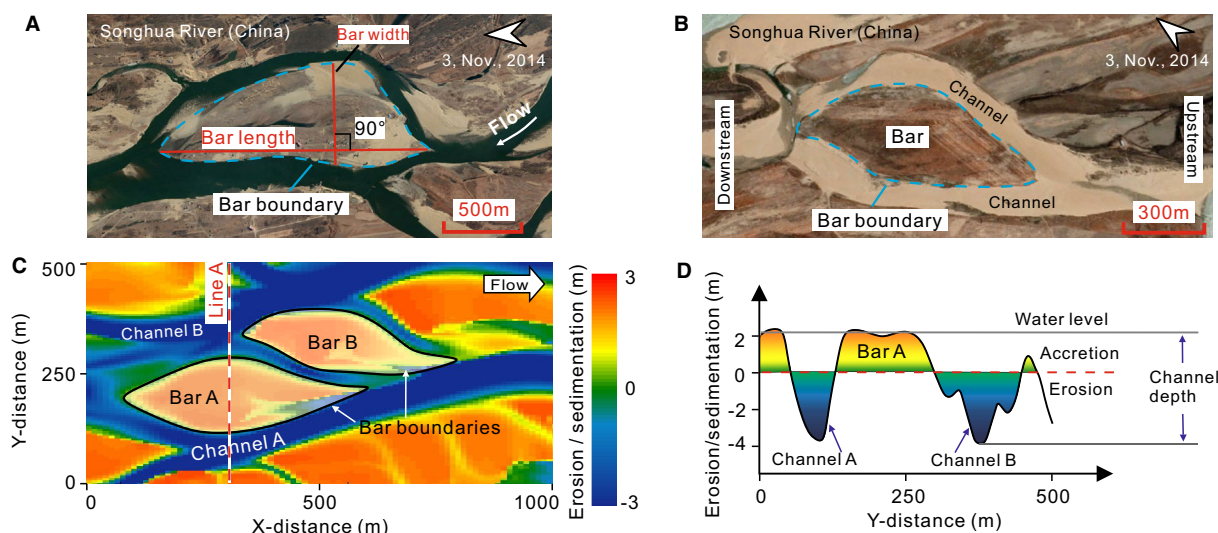
Fig. 1. Practical approach followed for placing the boundary between bars and channels. (A) Aerial photograph of the Songhua River, China (45°13'59"N, 43°10'E), at low flow stage. (B) Aerial photograph of the Songhua River, China (45°3'25"N, 124°59'21"E), presenting a mid-channel bar adjacent to channels with dry beds. Sandy channel beds are lighter coloured, whereas the vegetated bar appears darker. (C) Map of the amount of erosion and sedimentation of the riverbed of a modelled river, relative to the initial planar surface. The boundaries of two bars (labelled as 'Bar A' and 'Bar B') are shown as examples. (D) Cross-section of Line A in part (C).
