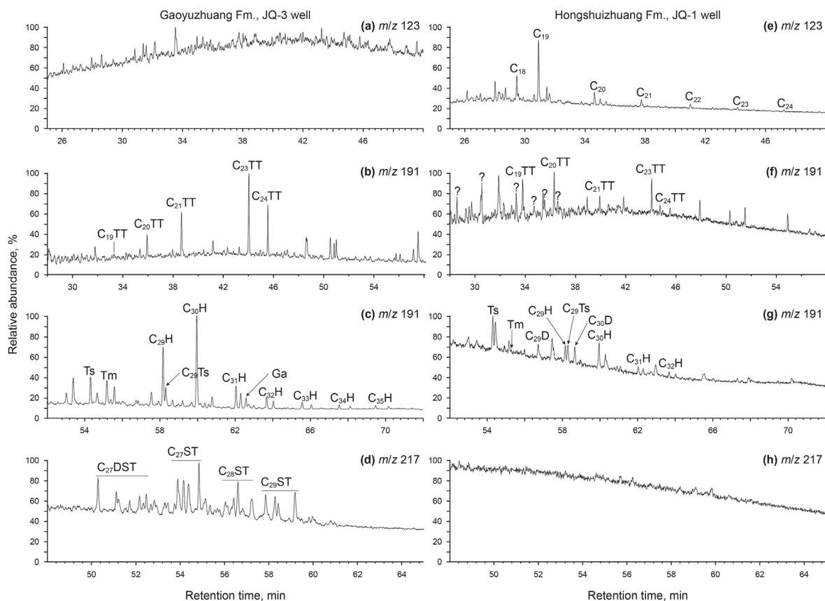
Fig. 5. Typical biomarker compositions of the representative samples of the Gaoyuzhuang and Hongshuizhuang formations. Notes: TT = tricyclic terpene; H = regular hopane; D = dihopane; DST = diasterane; ST = regular sterane; Ga = gammacerane.
