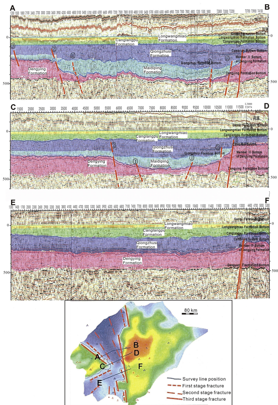
Fig. 14 Seismic profiles (A–B, C–D, and E–F) showing syndepositional faults developed during the Neoproterozoic and Early Paleozoic in Sichuan Basin.
