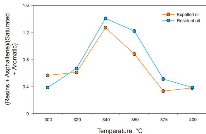
Fig. 8. Relationship between liquid product group component content and thermal evolution degree of the Lower Permian organic-rich oil shale in Tasmania, Australia (Data is from Lin et al., 2022).
