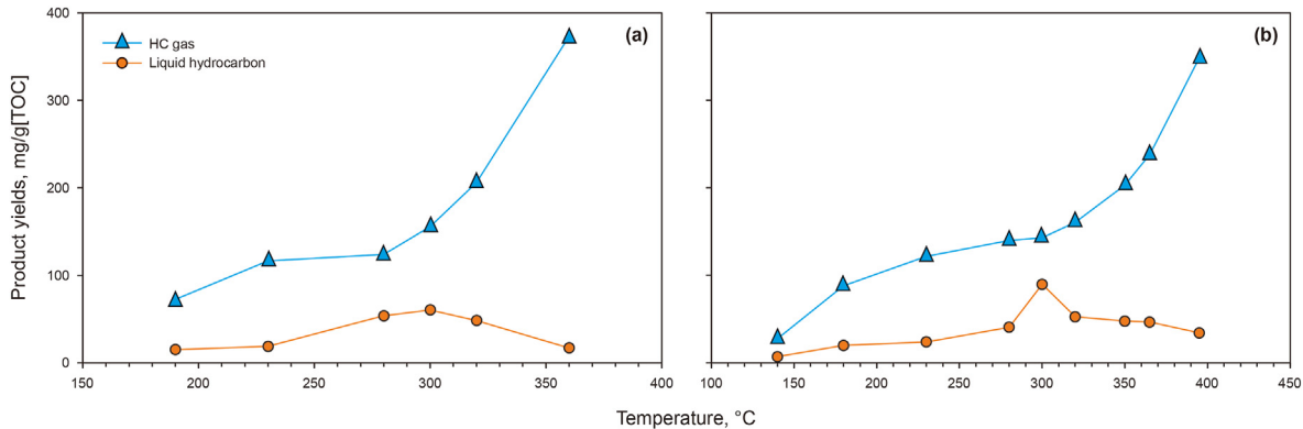
Fig. 5. Hydrus pyrolysis simulation experiment results from Jin (2000). Hydrocarbon generation evolution of samples rich in green algae (a); Hydrocarbon generation evolution of samples rich in cyanobacteria (b).
