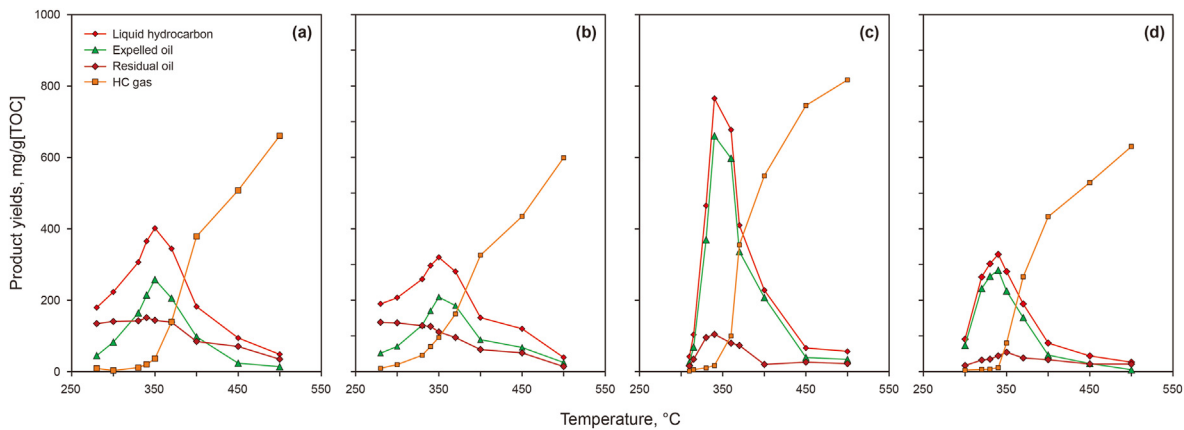
Fig. 4. Hydrus pyrolysis yields for the green algae-rich samples of the E 2-3a and the cyanobacteria-rich samples of the K 1q . Hydrocarbon generation evolution of sample Aj1 rich in green algae from the E 2-3a (a); Hydrocarbon generation evolution of sample Aj2 rich in green algae from the E 2-3a (b); Hydrocarbon generation evolution of sample Sc rich in Cyanobacteria from the K 1q (c); Hydrocarbon generation evolution of sample Pc1 rich in Cyanobacteria from the K 1q (d).
