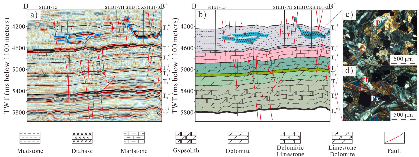
Fig. 8. Cross the No. 1 fault zone seismic section (a), the relevant geological schematic section (b), microscopic observation of the core at 6425–6430 m in well SHB1-3 (c and d).
