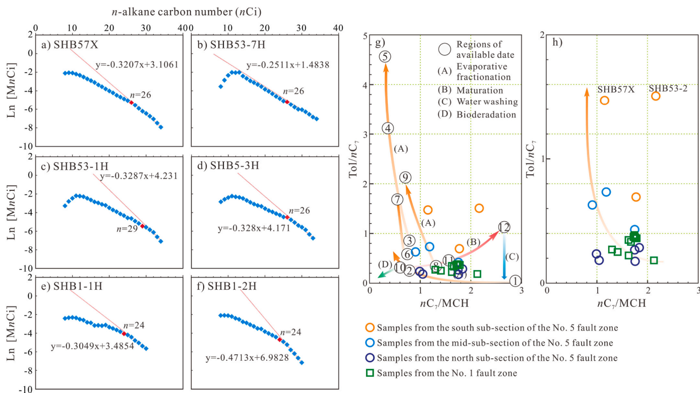
Fig. 13. Cross-plots indicating the differential evaporation fractionation of oils from the Shunbei oilfield. Log of mole concentration of \text{C}_5 – \text{C}_{35} n -alkanes versus carbon numbers (a–f), \text{Tol}/n\text{C}_7 versus n\text{C}_7/\text{MCH} (g and h) (refer to Thompson, 1987).
