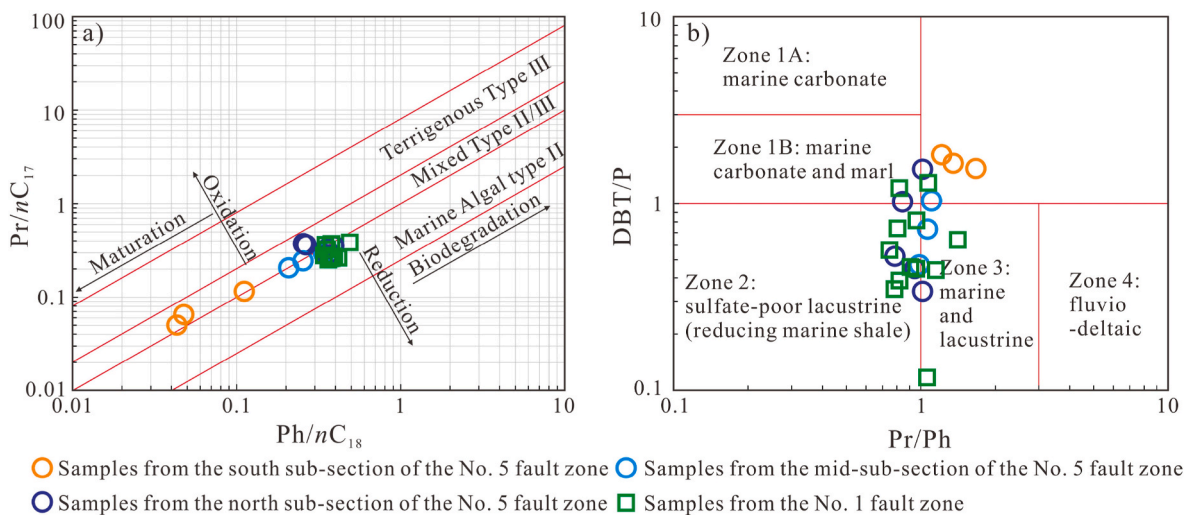
Fig. 10. Cross-plots identify sedimentary environments. a) phytane (Ph)/ n -C 18 versus pristane (Pr)/ n -C 17 (refer to Shanmugam, 1985 ); b) pristane (Pr)/phytane (Ph) versus dibenzothiophene (DBT)/dibenzothiophene (P) (refer to Hughes et al., 1995 ).
