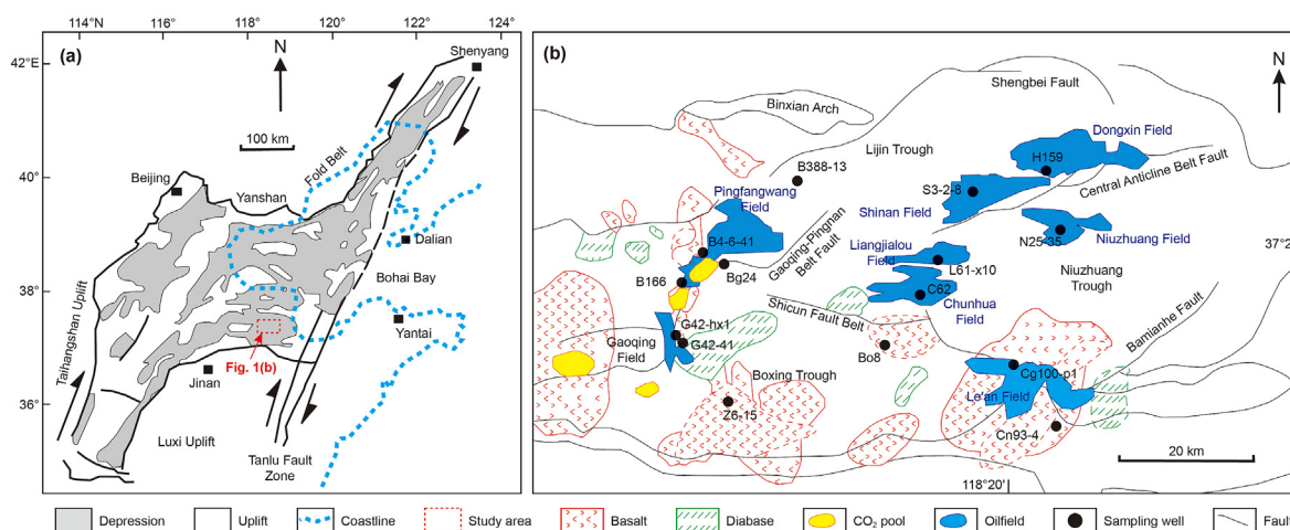
Fig. 1. Location map of the Dongying Depression. (a) Structural map of the Bohai Bay Basin and location of the Dongying Depression (modified from Li et al., 2024); (b) structural map of the Dongying Depression showing distribution of faults, CO 2 pools, igneous rocks and oilfields (modified from Zhang et al., 2009, and based on maps from Jin et al., 2002).
