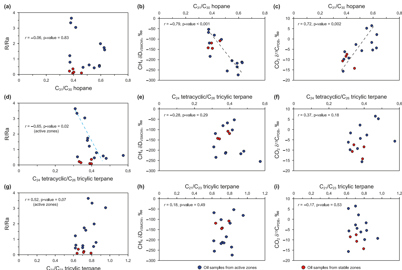
Fig. 9. Correlation diagrams of C_{31}/C_{30} hopane versus (a) R/Ra , (b) \delta^{2}H_{CH_4} and (c) \delta^{13}C_{CO_2} , C_{24} tetracyclic/ C_{26} tricyclic terpene versus (d) R/Ra , (e) \delta^{2}H_{CH_4} and (f) \delta^{13}C_{CO_2} , and C_{21}/C_{23} tricyclic terpene versus (g) R/Ra , (h) \delta^{2}H_{CH_4} and (i) \delta^{13}C_{CO_2} .
