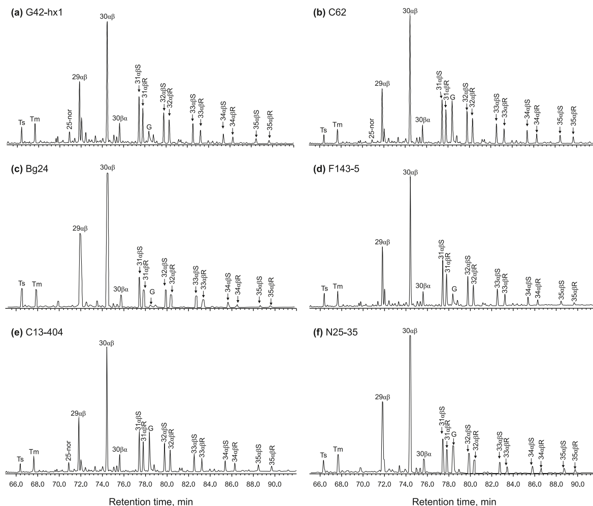
Fig. 8. Partial m/z 191 mass chromatograms of representative crude oils from the Dongying Depression. Peak assignments define stereochemistry at C-22 (S and R); \alpha\beta and \beta\alpha denote 17\alpha(\text{H}) -hopanes and 17\beta(\text{H}) -moretanes, respectively; Ts = \text{C}_{27}18\alpha(\text{H}) , 22, 29, 30-trisnorhopane; Tm = \text{C}_{27}17\alpha(\text{H}) , 22, 29, 30-trisnorhopane; 25-nor = \text{C}_{29} 25-norhopane; G: gammacerane.
