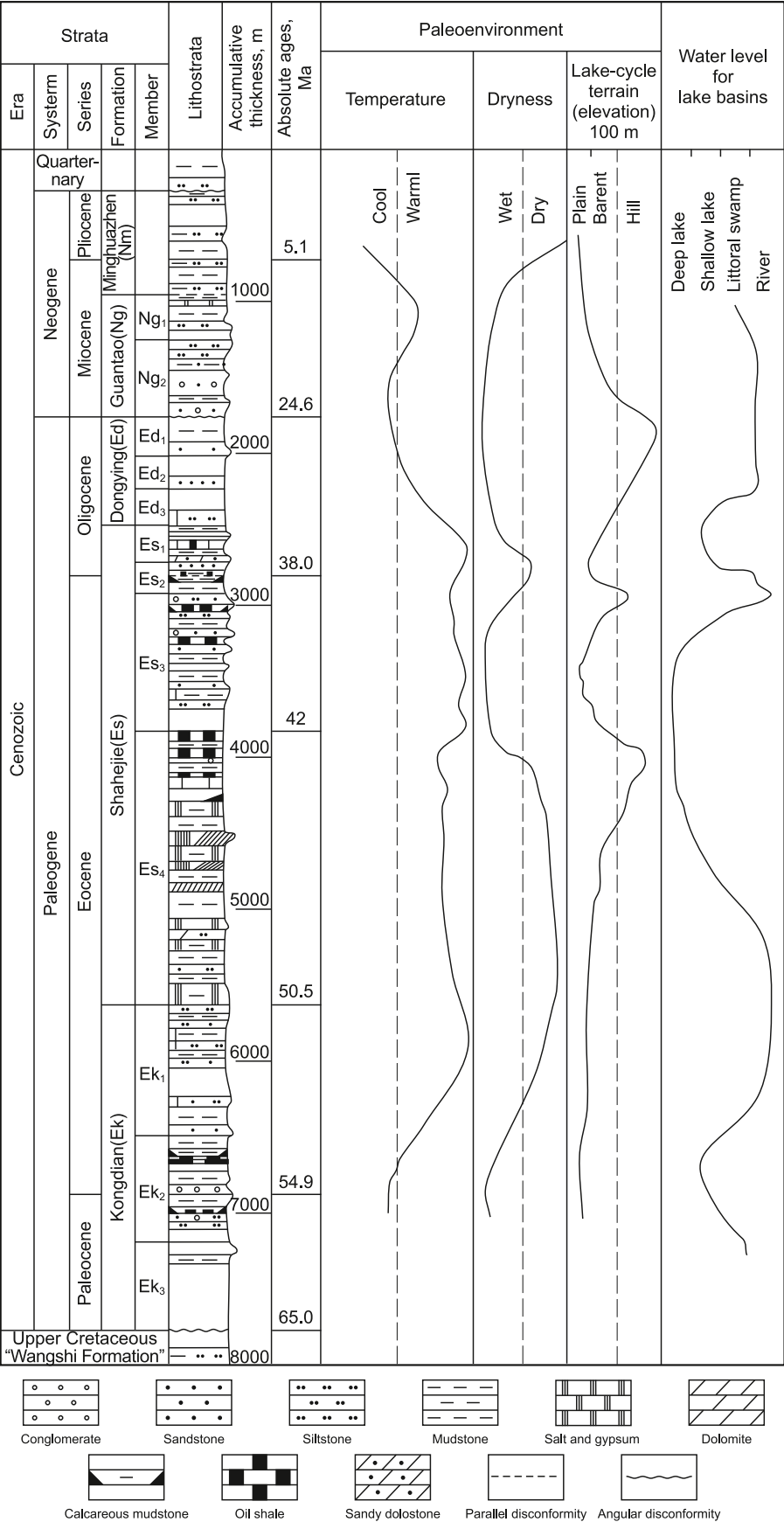
Fig. 2. Generalized Cenozoic stratigraphy of the Dongying Depression showing lithology and paleoenvironment of each unit (modified from Group of Shengli Oil Field Compiling Petroleum Geology, 1993).
