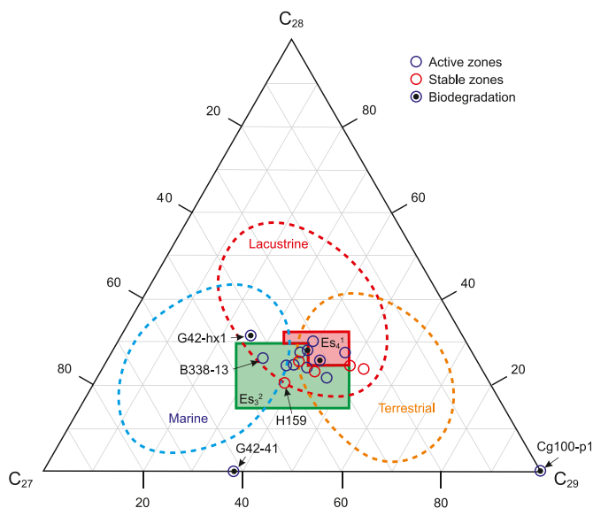
Fig. 7. Ternary diagram showing the relative distributions of C_{27} , C_{28} and C_{29} \alpha\alpha\alpha (20R) steranes. Ranges of source rocks from Es_3 (green square) and Es_4 (red square) are modified from Tan et al. (2002). Ranges of terrestrial (yellow dashed lines), lacustrine (red dashed lines) and oceanic (blue dashed lines) environments are based on Peters and Moldowan (1993).
