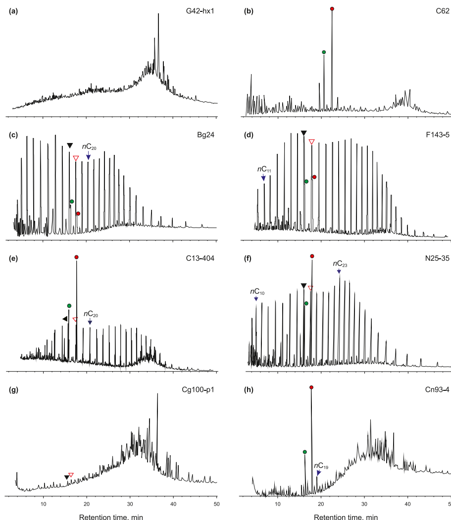
Fig. 4. Gas chromatograms of representative crude oils from the Dongying Depression. The peak labels denote the carbon number of n -alkanes; green circle denotes Pr; red circle denotes Ph; red triangle denotes n -C 18 ; black triangle denotes n -C 17 .
