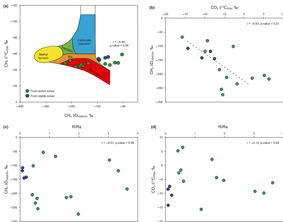
Fig. 3. Correlation diagrams (a) between \delta\text{D}_{\text{CH}_4} and \delta^{13}\text{C}_{\text{CH}_4} , (b) between \delta\text{D}_{\text{CH}_4} and \delta^{13}\text{C}_{\text{CO}_2} , (c) between \delta\text{D}_{\text{CH}_4} and \text{R/Ra} , and (d) between \delta^{13}\text{C}_{\text{CO}_2} and \text{R/Ra} in gas from the Dongying Depression. The isotopic compositions for different types of methane in (a) are modified from Whiticar (1990). “r” is short for Pearson correlation coefficient.
