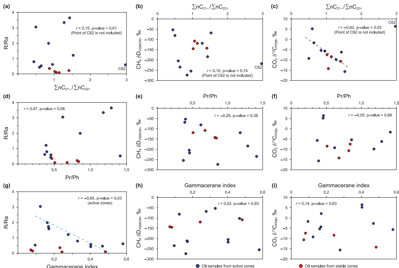
Fig. 5. Correlation diagrams of \Sigma nC_{21-}/\Sigma nC_{22+} versus (a) R/Ra , (b) D_{CH_4} and (c) \delta^{13}C_{CO_2} , Pr/Ph versus (d) R/Ra , (e) D_{CH_4} and (f) \delta^{13}C_{CO_2} , and gammacerane index versus (g) R/Ra , (h) D_{CH_4} and (i) \delta^{13}C_{CO_2} .
