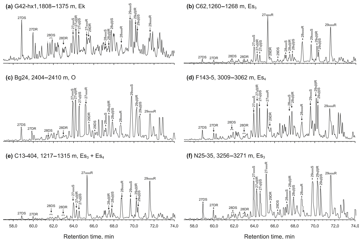
Fig. 6. Partial m/z 217 mass chromatograms of representative crude oils from the Dongying Depression. Peak assignments define stereochemistry at C-20 (S and R); \alpha\alpha\alpha and \alpha\beta\beta denote 5 \alpha (H), 14 \alpha (H), 17 \alpha (H)-steranes and 5 \alpha (H), 14 \beta (H), 17 \beta (H)-steranes, respectively; D = 13 \beta (H), 17 \alpha (H)-diasteranes.
