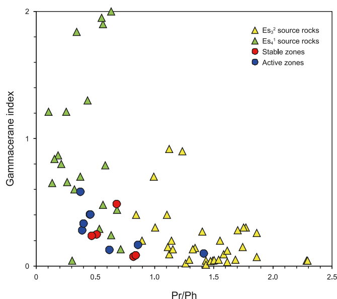
Fig. 10. Variation of Pr/Ph with gammacerane index in oils (blue and red circles) and source rocks (yellow and green triangles) in the Dongying Depression. The source rock data are based on the results from Zhu and Jin (2003).
