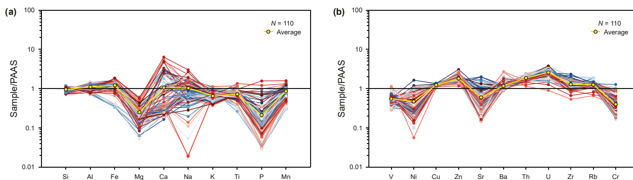
Fig. 3. Standardized spider web map of elements. (a) Major elements map of the lower Mbr. WC Fm. (b) Trace element map of the lower Mbr. WC Fm. mudstones standardized by PAAS (PAAS data from Hu and Gao, 2008). The yellow dots were the average values of 110 samples standardized by PAAS.
