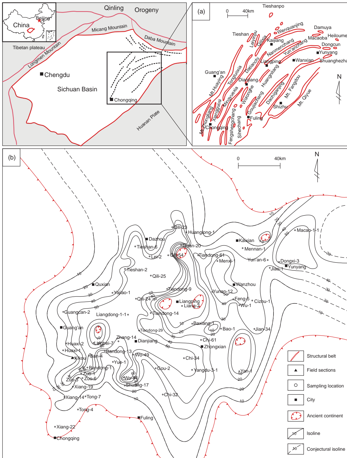
Fig. 1 (a) The tectonic map of Eastern Sichuan Basin (b) The isopach map of the Huanglong Formation
