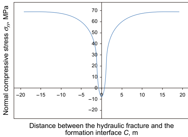
Fig. 12 Normal compressive stress at the formation interface at a dip angle of 0^\circ
