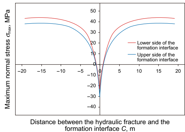
Fig. 10 Maximum normal stress at the formation interface at a dip angle of 0^\circ
