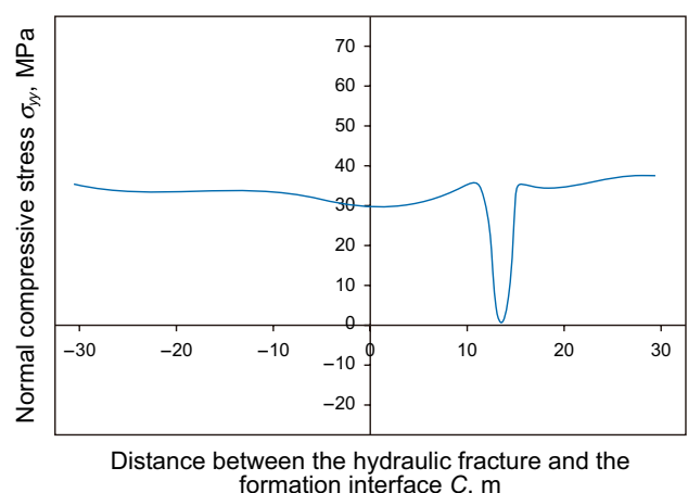
Fig. 15 Normal compressive stress at the formation interface at a dip angle of 45^\circ
