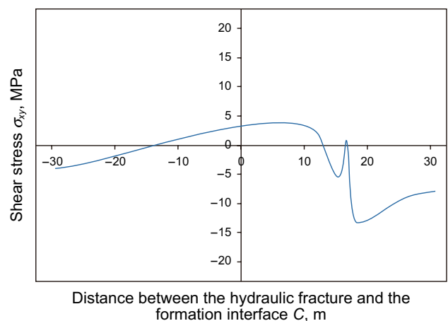
Fig. 16 Shear stress at the formation interface at a dip angle of 45^\circ
