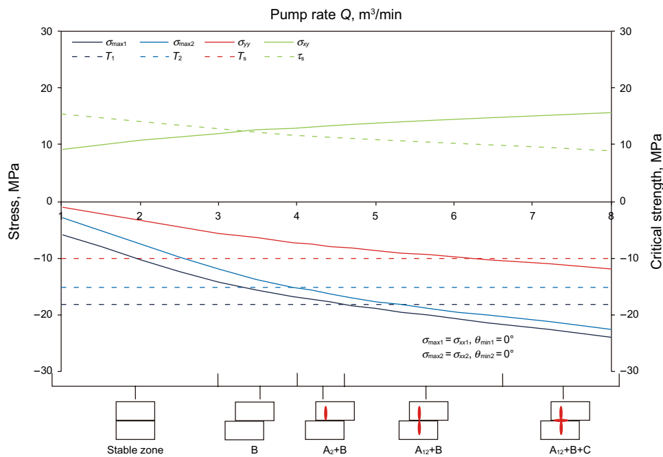
Fig. 21 Shear and tensile failure modes of the formation interface under the impact of hydraulic fracture propagation near the formation interface at different pump rates
