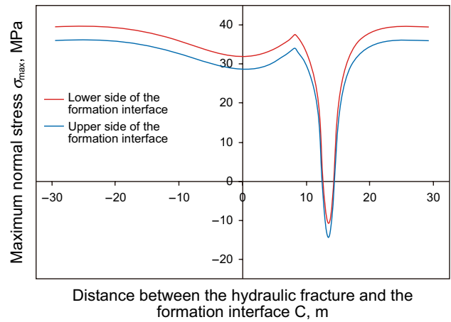
Fig. 14 Maximum normal stress at the formation interface at a dip angle of 45^\circ
