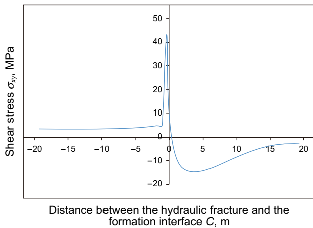
Fig. 13 Shear stress at the formation interface at a dip angle of 0^\circ
