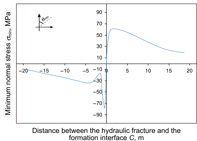
Fig. 11 Direction of minimum normal stress at the formation interface at a dip angle of 0^\circ
