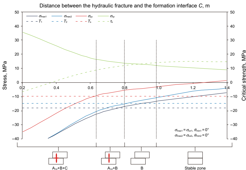
Fig. 20 Shear and tensile failure modes of the formation interface under the impact of hydraulic fracture propagation near the formation interface at different distances between the hydraulic fracture and the formation interface
