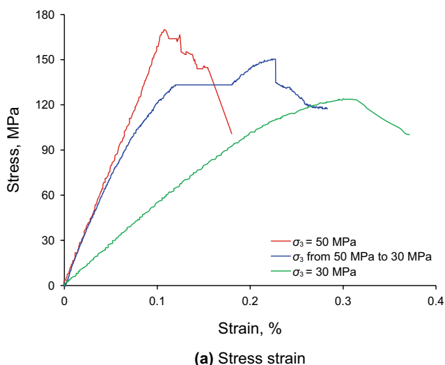
Fig. 9 Comparison of strength property in conventional and unloading conditions
