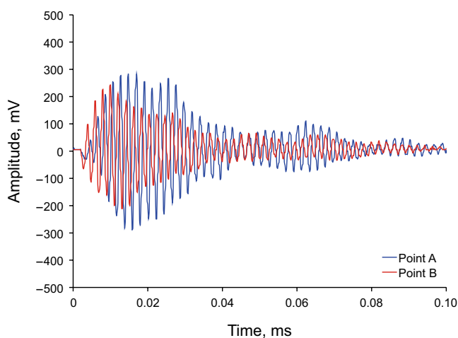
(b) Ultrasonic wave at Point A and Point B
