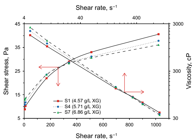
Fig. 6 Effect of XG concentration on shear stress and viscosity of CGA fluids at 0.34 g/L SDBS
