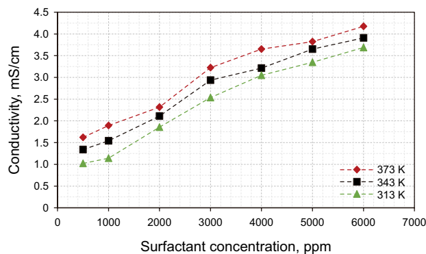
Fig. 14 Conductivity diagram of surfactant solutions at different concentrations
