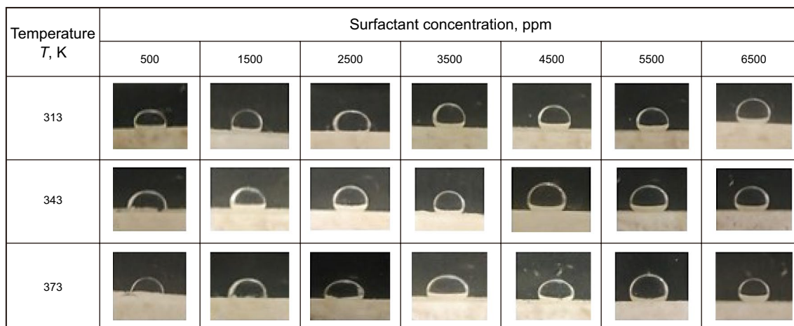
Fig. 13 Liquid droplet images on the treated sections in surfactant solutions at different concentrations and at different temperatures of 313, 343 and 373 K and treatment time equal to 240 min
