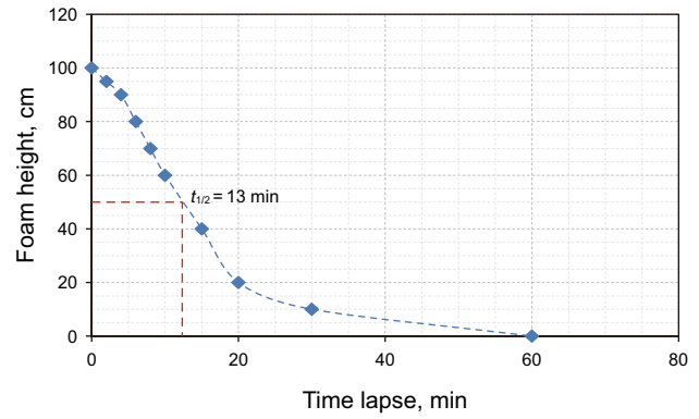
Fig. 16 Foam height diagram over time
