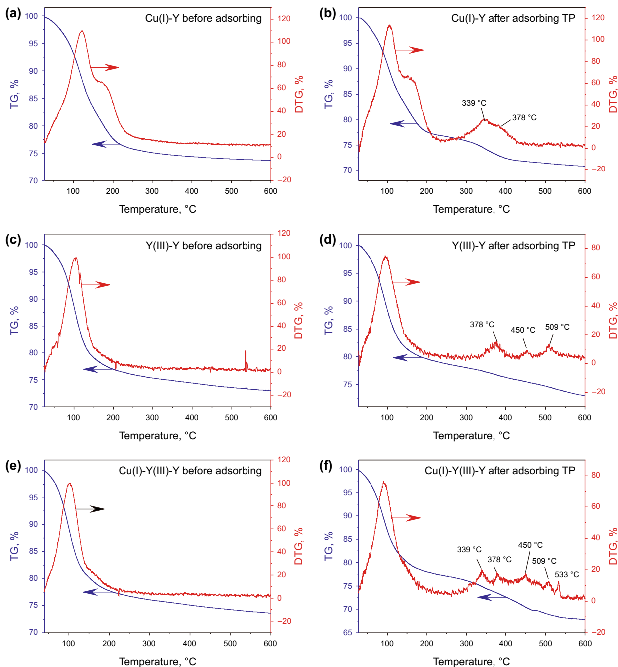
Fig. 4 TG and DTA curves of Cu(I)-Y, Y(III)-Y and Cu(I)-Y(III)-Y before and after adsorbing TP
