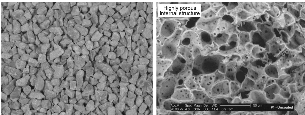
Fig. 4 Photograph showing the angularity of a 1.25 specific gravity ULW proppant (Rickards et al. 2006)
