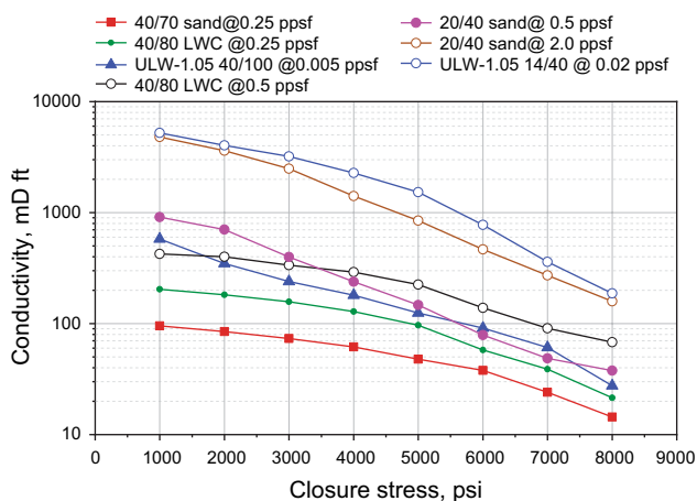
Fig. 9 Proppant conductivity vs. closure stress (Brannon and Starks 2009)
