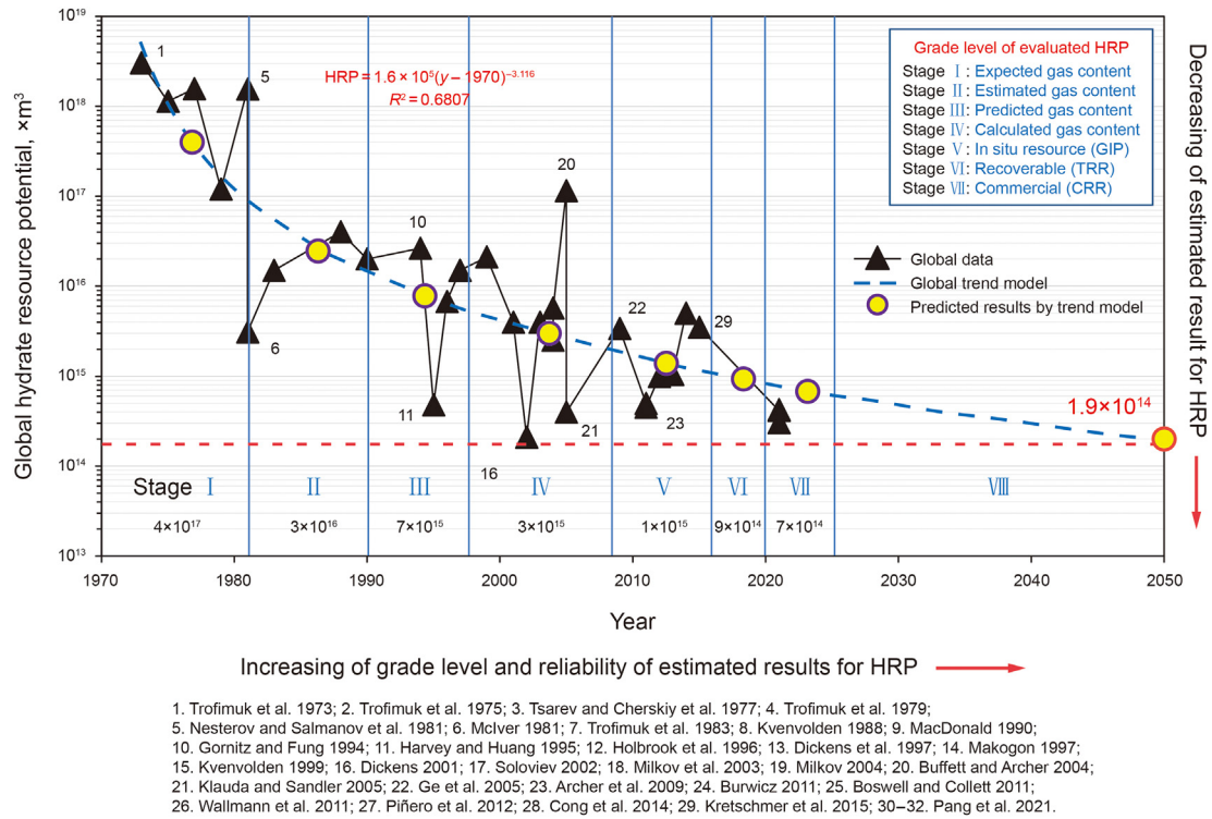
Fig. 4. Variation of global 29 estimates of NGH resource with time (modified from Pang et al., 2021). A trend model was established to predict the NGH TRR at seventh stages (2021–2025) and CRR in 2050 according to the lower red asymptote. The values of NGH resource estimates decrease but the grade level and reliability increase.
