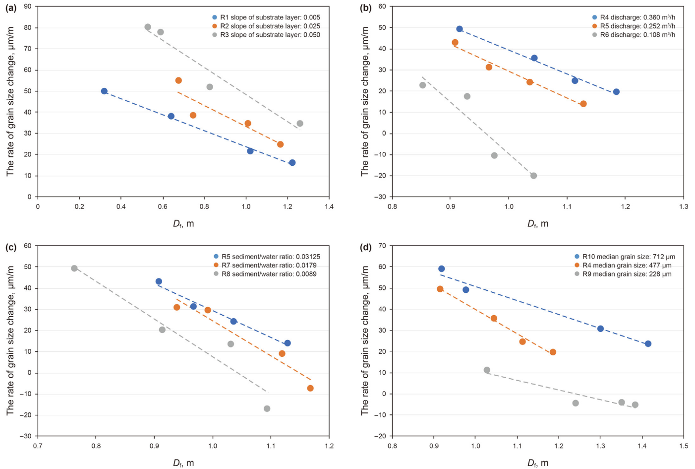
Fig. 7. The rate of grain size change along the foreset bedding for experiments. The rate of grain size change along the foreset bedding shows a decreasing trend as the D_f gradually increases. It also decreases with the decrease of slope of substrate layer, discharge, sediment/water ratio and median grain size of sediment supplied.
