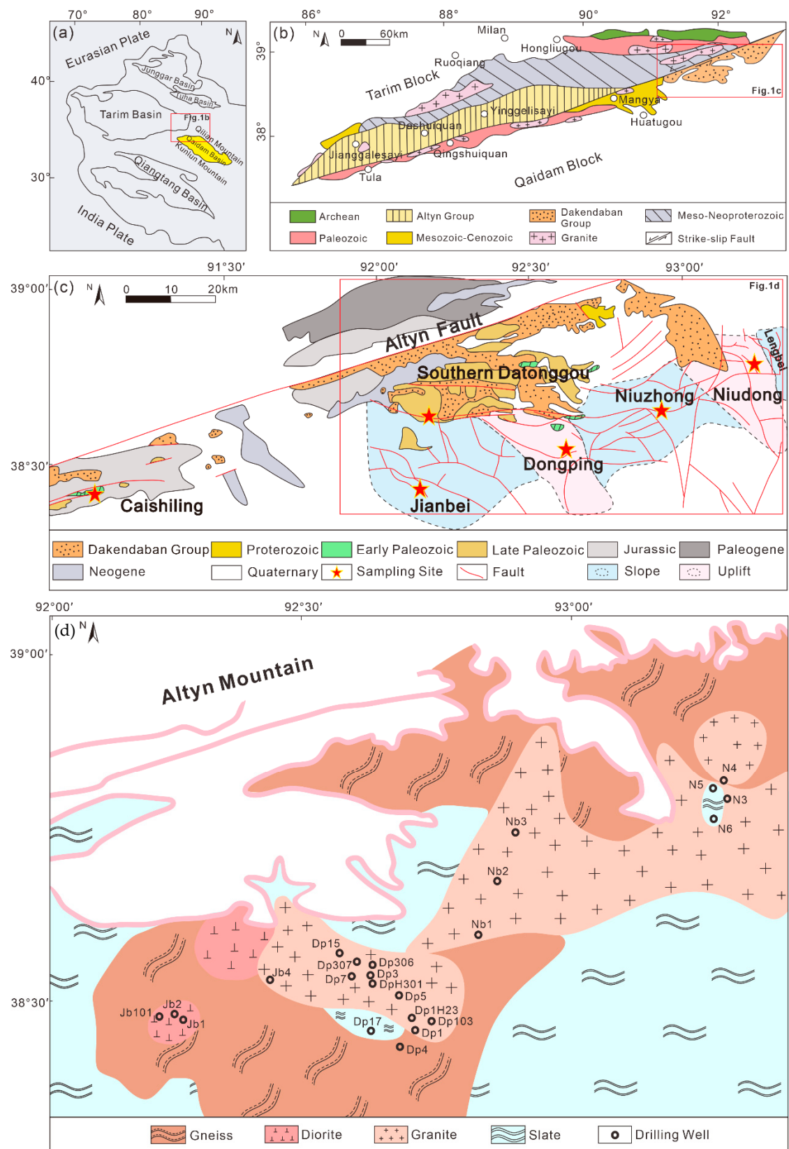
Figure 1. (a) Geological sketch map of the Qaidam region. (b) Tectonic sketch map of the Altyn orogenic belt (modified after Wu et al. [57] and Niu et al. [58]). (c) Sampled areas analyzed in this study (modified after Niu et al. [58]). (d) Lithological distribution and the drilling well locations of Qinghai oilfield in Qaidam Basin.
