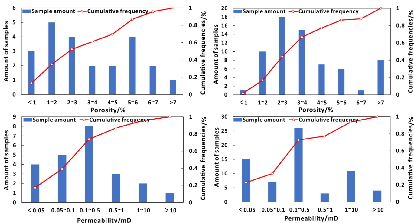
Figure 11. Physical properties of granite and granitic gneiss. (a) The distribution of porosity of granite; (b) the distribution of porosity of granitic gneiss; (c) the distribution of permeability of granite; (d) the distribution of permeability of granitic gneiss.
