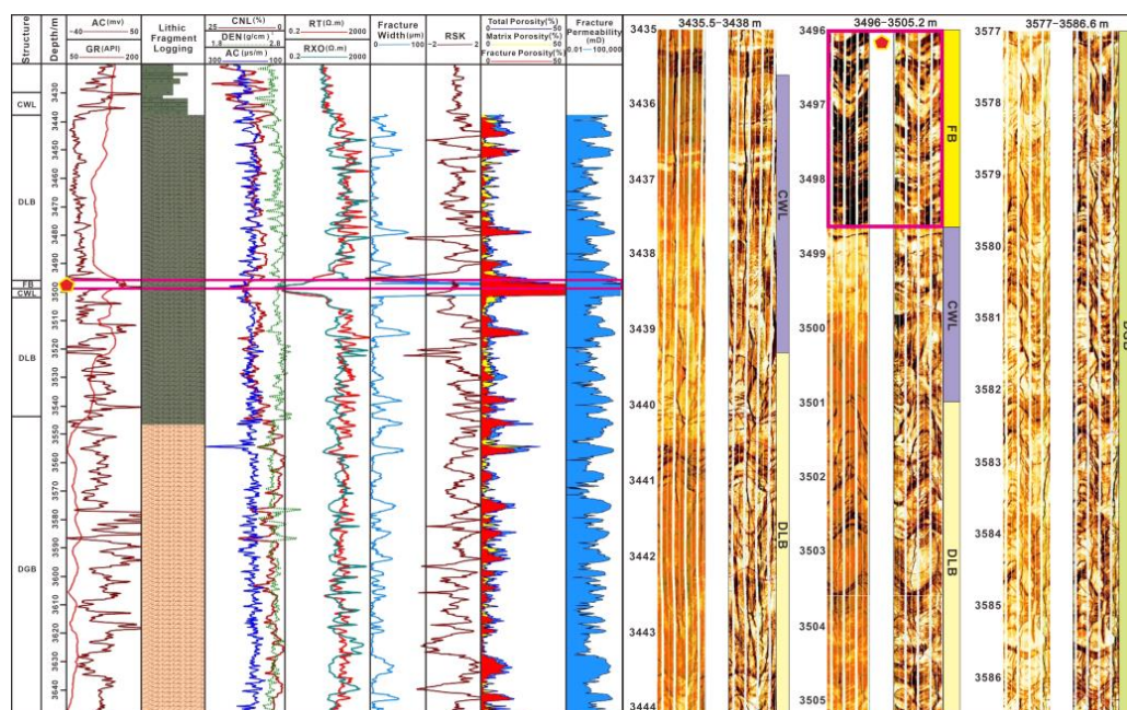
Figure 13. Identification of fault belts and characterization of their physical properties from the logging dataset. CWL: complete weathering layer, FB: fault belt, DLB: dissolution belt, DGB: disintegration belt.
