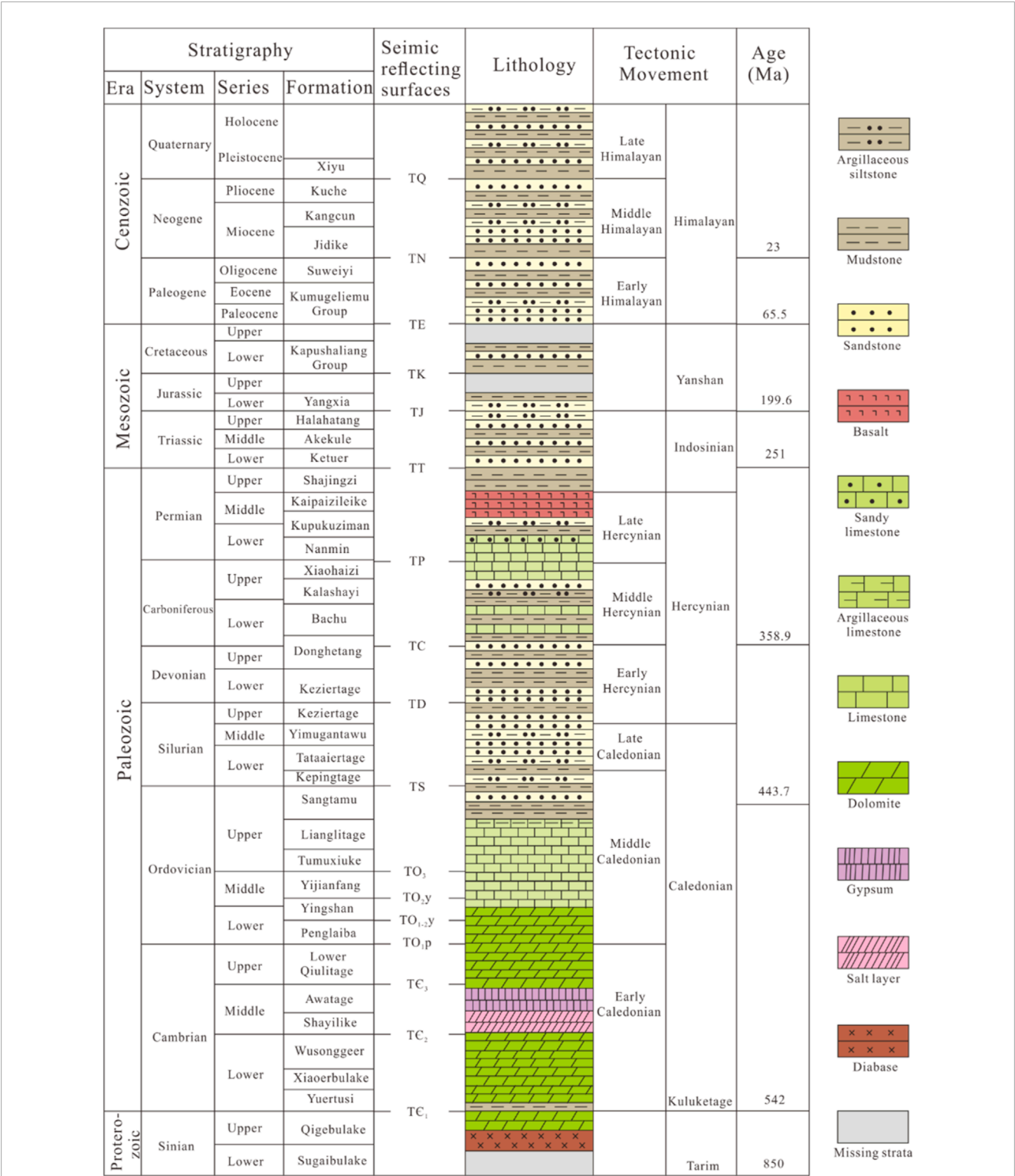
FIGURE 2 Chart showing the Tarim Basin stratigraphy, the seismic reflecting surfaces (horizons), and the timing of regional tectonic movements [modified from Deng et al. (2019), Neng et al. (2022)].
