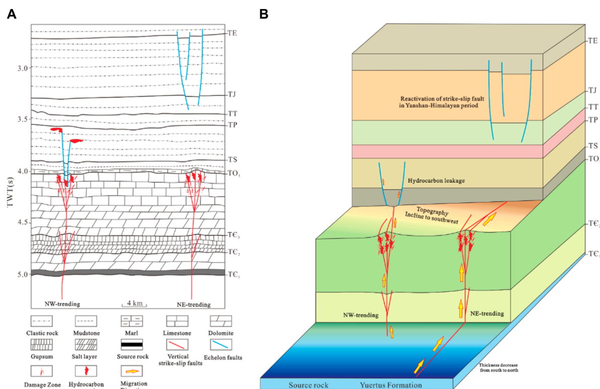
FIGURE 16 (A) Reservoir modeling and (B) the model of hydrocarbon differential enrichment in the Tabei Uplift.
