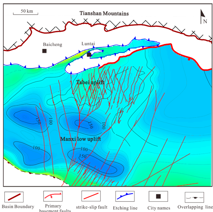
FIGURE 15 Distribution of source rocks of the Lower Cambrian Yuertus Formation around the Tabei Uplift.
