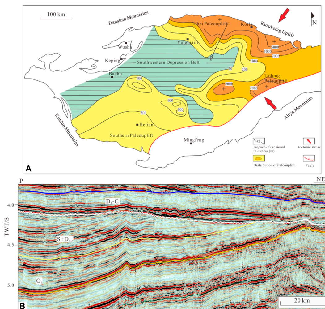
FIGURE 11 (A) The erosion thickness distribution of unconformity in the Devonian and the prediction of tectonic stress [modified from Lin et al. (2012), He et al. (2016)] and (B) seismic profile of the Devonian strata denudation in the Tabei Uplift.
