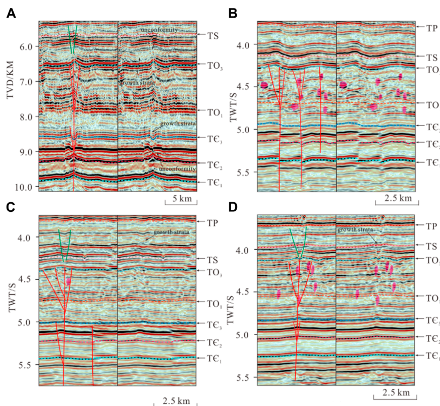
FIGURE 7 Typical 3D seismic profiles of multistage evolution (for location, see Figures 1B, 6).
