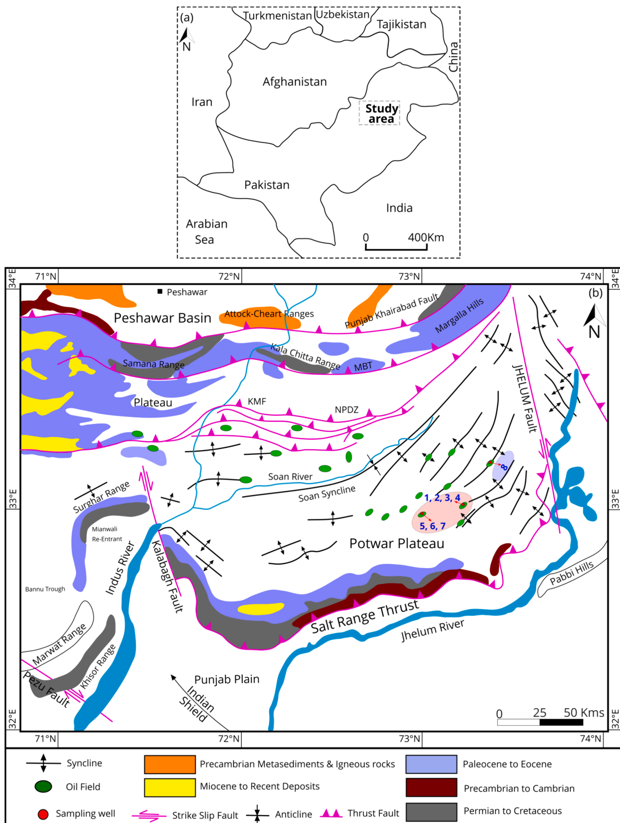
Fig. 1. Map showing the location of the study area (a), geological map showing the studied crude oils and structural features of PTB, Pakistan (b) (after modified wandrey et al. 2004 ; and references therein).
