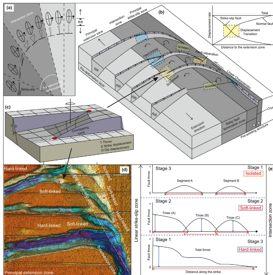
Fig. 18. Transtensional fault linkage evolution model. (a) Incremental horizontal strain ellipses illustrating principal horizontal shortening and extensions across the deformation zone (modified after Mouslopoulou et al., 2007). (b) 3D model of the transtensional fault linkage evolution in different principal deformation zones. The curve graph illustrates the relationship between the strike-slip displacement rate and the extension displacement rate. (c) 3D model of the rotational relay ramp in the overlapping zone (modified after Fossen and Rotevatn, 2016). (d) 3D stereogram of the linkage process of the transtensional faults (result in Model 2). (e) Plot showing the transtensional evolution statistics: fault throws along strike statistics.
