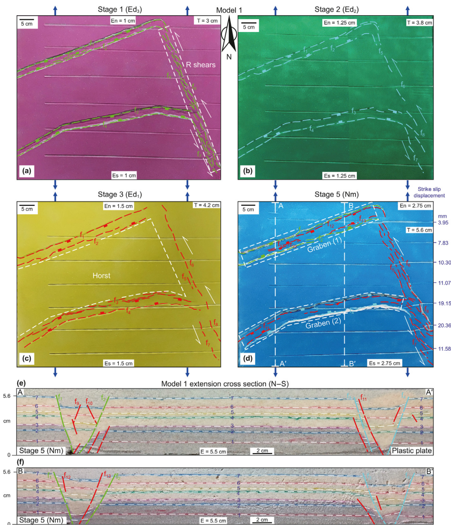
Fig. 10. (a)–(d) Top views (photographs and line drawings) of different stages of Model 1 showing the evolution of the structural zone at different extension stages. (e) and (f) N–S cross-section interpretations (photographs and line drawings) of the final stage of Model 1 representing the deformation styles (for cross-section locations, see Fig. 10(d)). Ed 3 : third Mbr of the Dongying Fm in Oligocene; Ed 2 : second Mbr of the Dongying Fm in Oligocene; Ed 1 : first Mbr of the Dongying Fm in Oligocene; Nm: Minghuazhen Fm in Pliocene; En and Es represent the extension from the north and south direction; T represents the total thickness of the sand layer; and the blue arrow represents the direction of extension.
