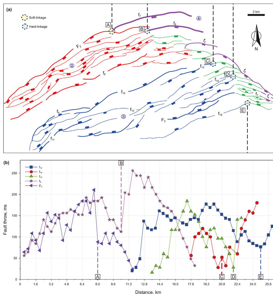
Fig. 17. Fault throw statistics of normal and transtensional faults. (a) Structural zone plan map; legend consistent with Fig. 5(a). (b) Plot showing the fault throw statistics of the five faults.
