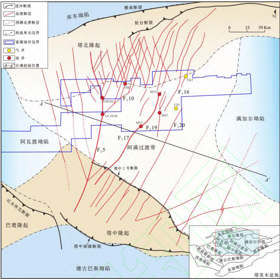
图 1 富满油田区域构造位置及邻区下古生界主要断裂分布 Fig.1 Regional structural location of Fuman Oilfield and Distribution of main faults of Lower Paleozoic in adjacent area
