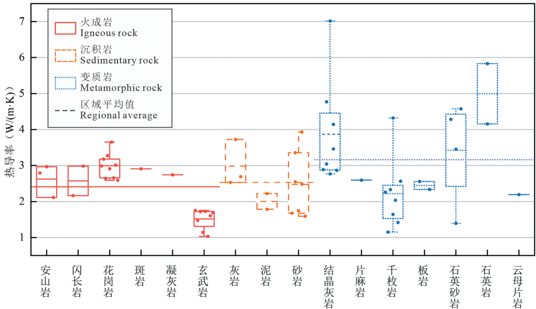
图 2 海南岛野外露头岩性热导率统计图 Fig. 2 Statistical chart of thermal conductivity of outcrop lithology in Hainan Island
