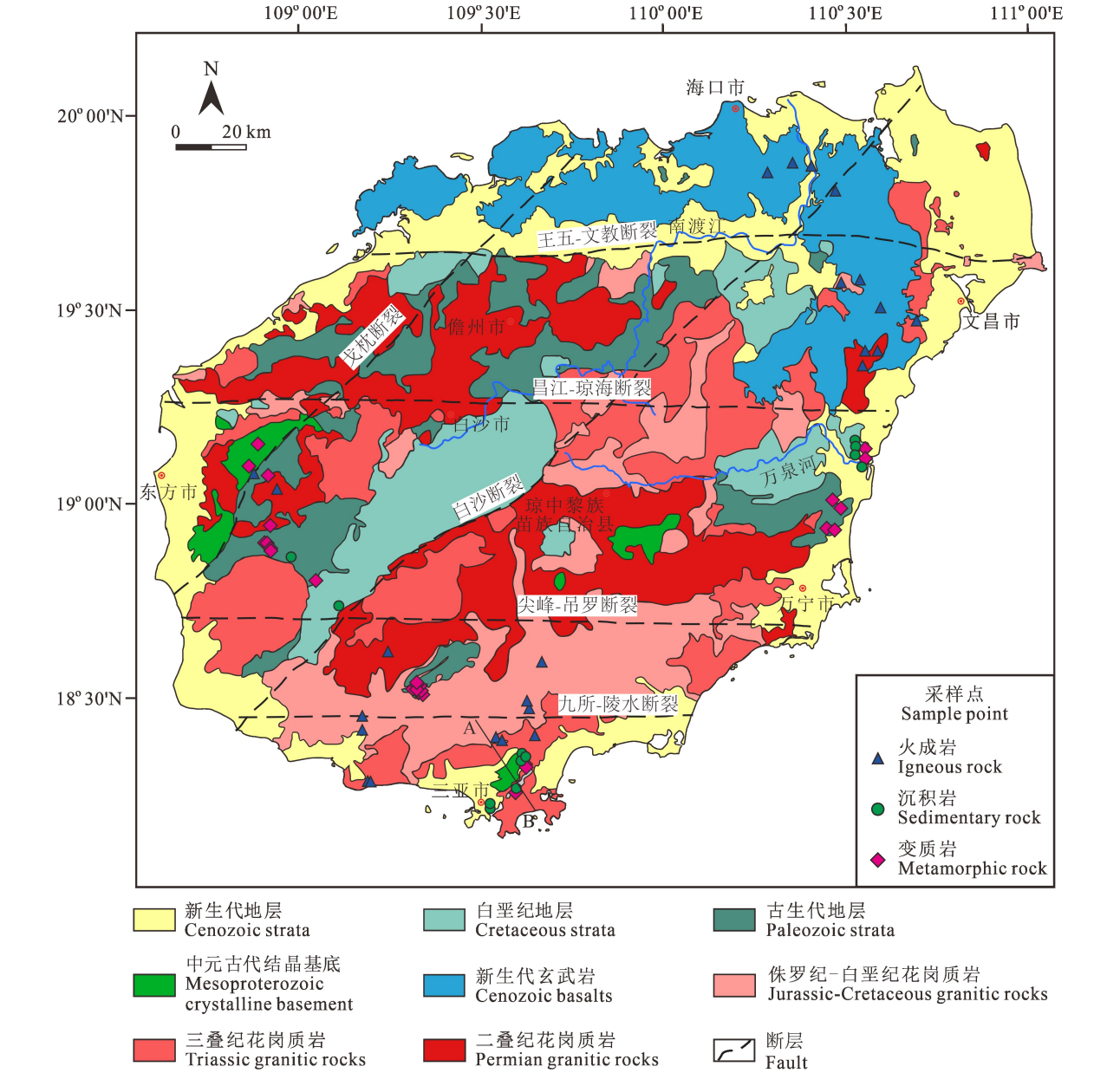
图 1 海南岛地质简图及采样点位(据张磊等,2022 修改) Fig. 1 Geological map and sample points of Hainan Island (modified from Zhang Lei et al. , 2022)
