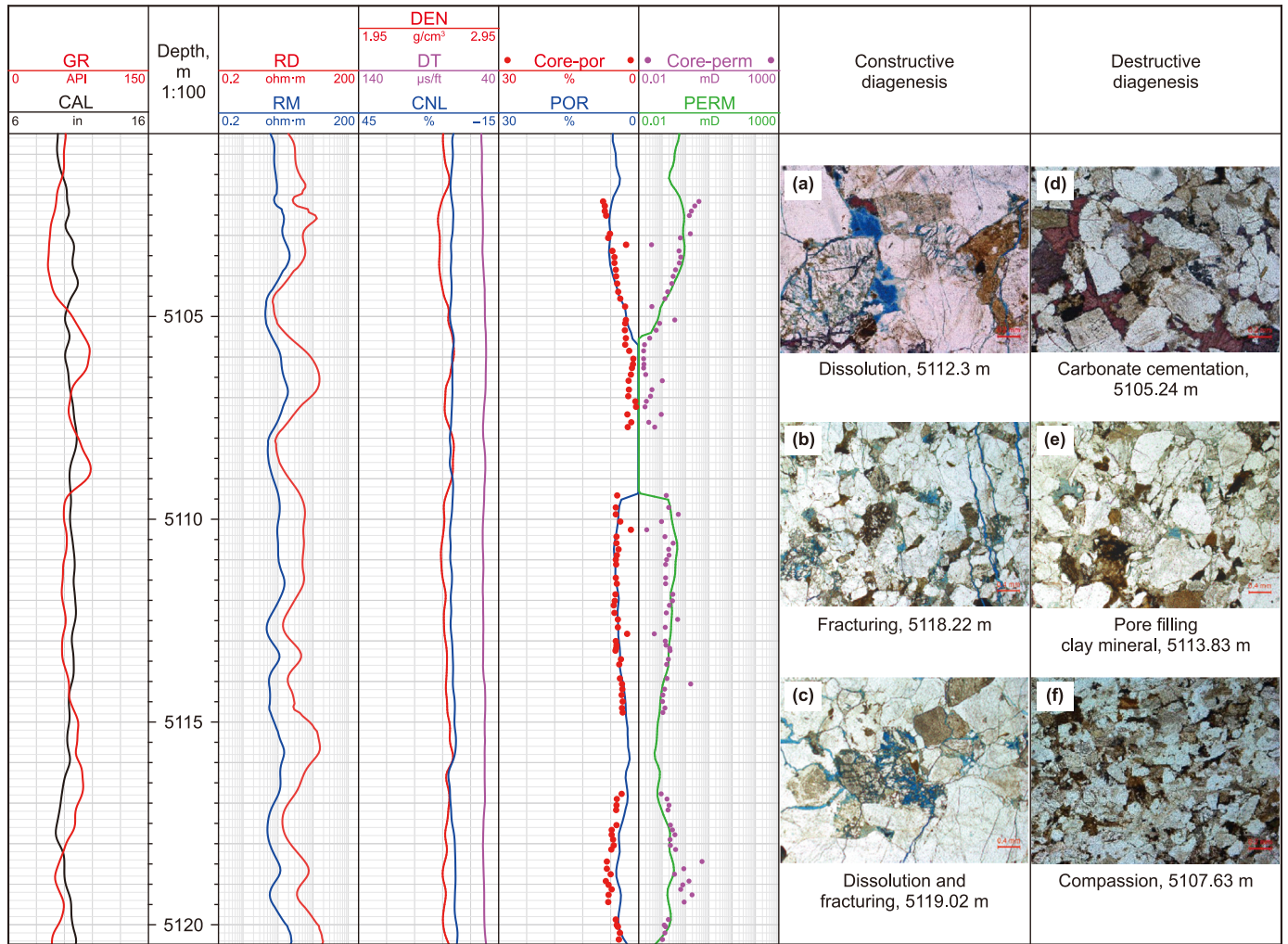
Fig. 11. The relationship between the physical properties and the diagenesis of Jurassic Ahe Formation in Kuqa Depression.
