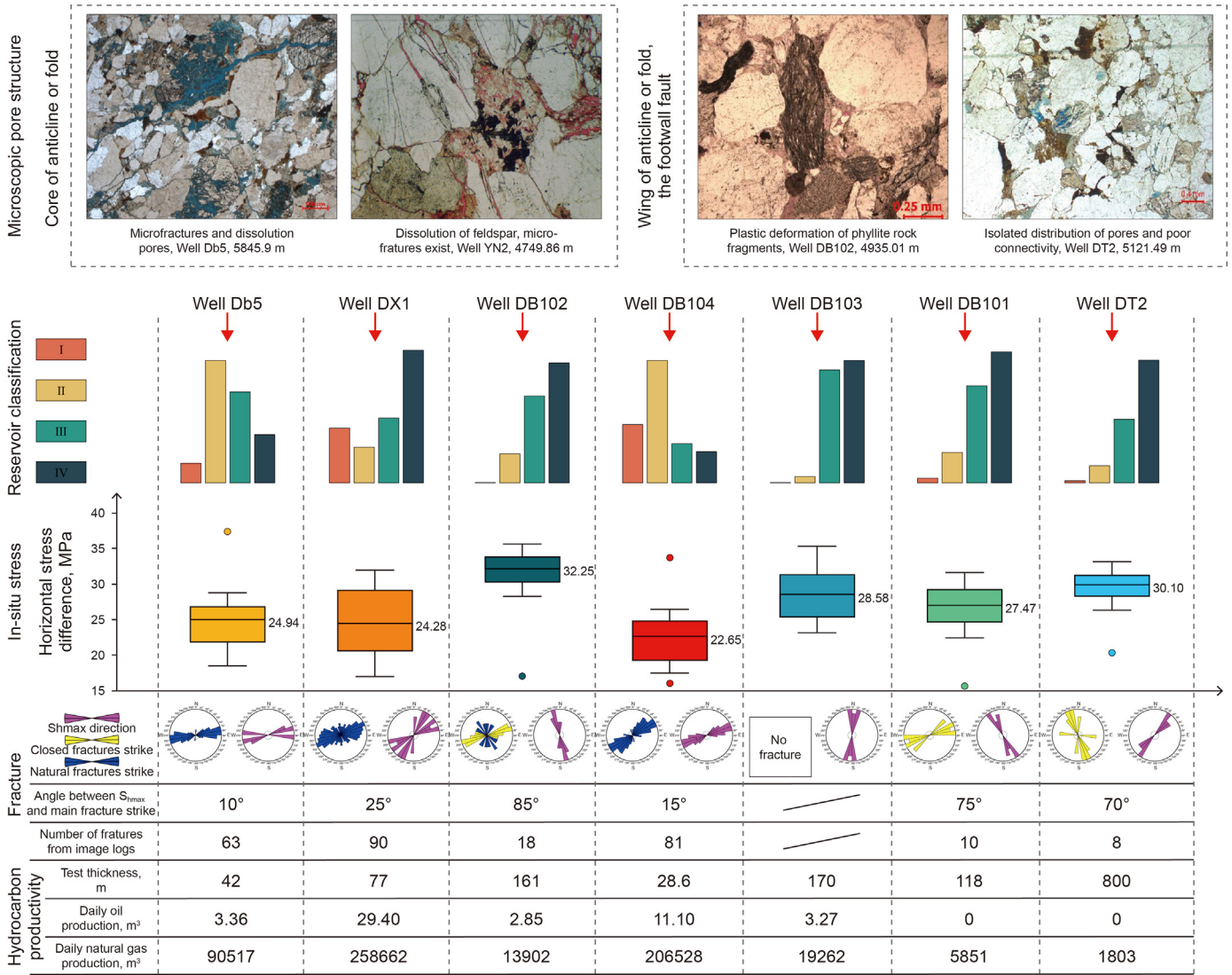
Fig. 20. Cross section of Dibei block and corresponding single well reservoir characteristics of Jurassic Ahe Formation in Kuqa Depression.
