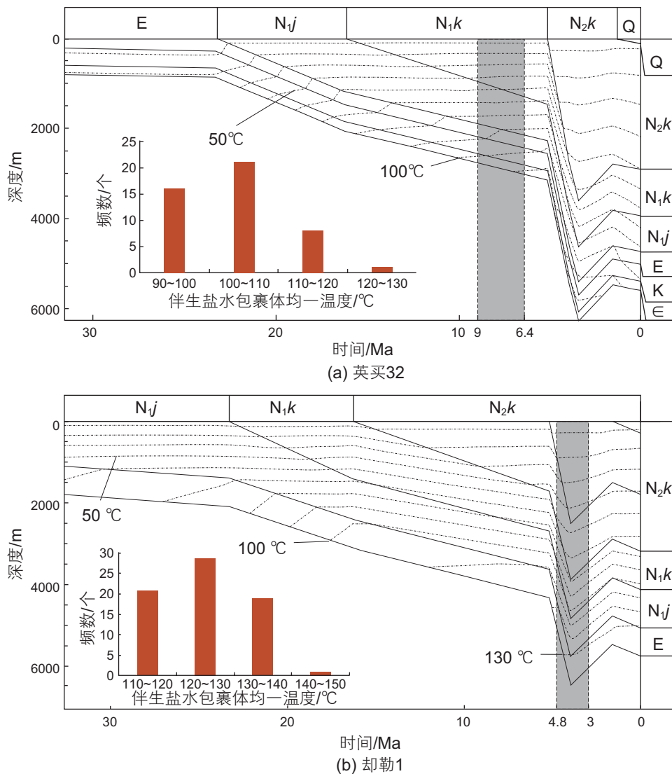
图 8 英买 32 井、却勒 1 井盐水包裹体均一温度分布及埋藏史、热史分析 Fig. 8 Analysis of homogeneous temperature distribution and burial history and thermal history of salt-water inclusions in the Yingmai-32 Well(a) and the Quele-1 Well(b)
